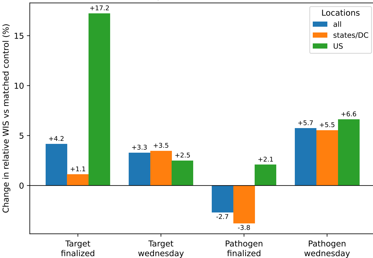
Kinsa vs no covariate · negative is better
