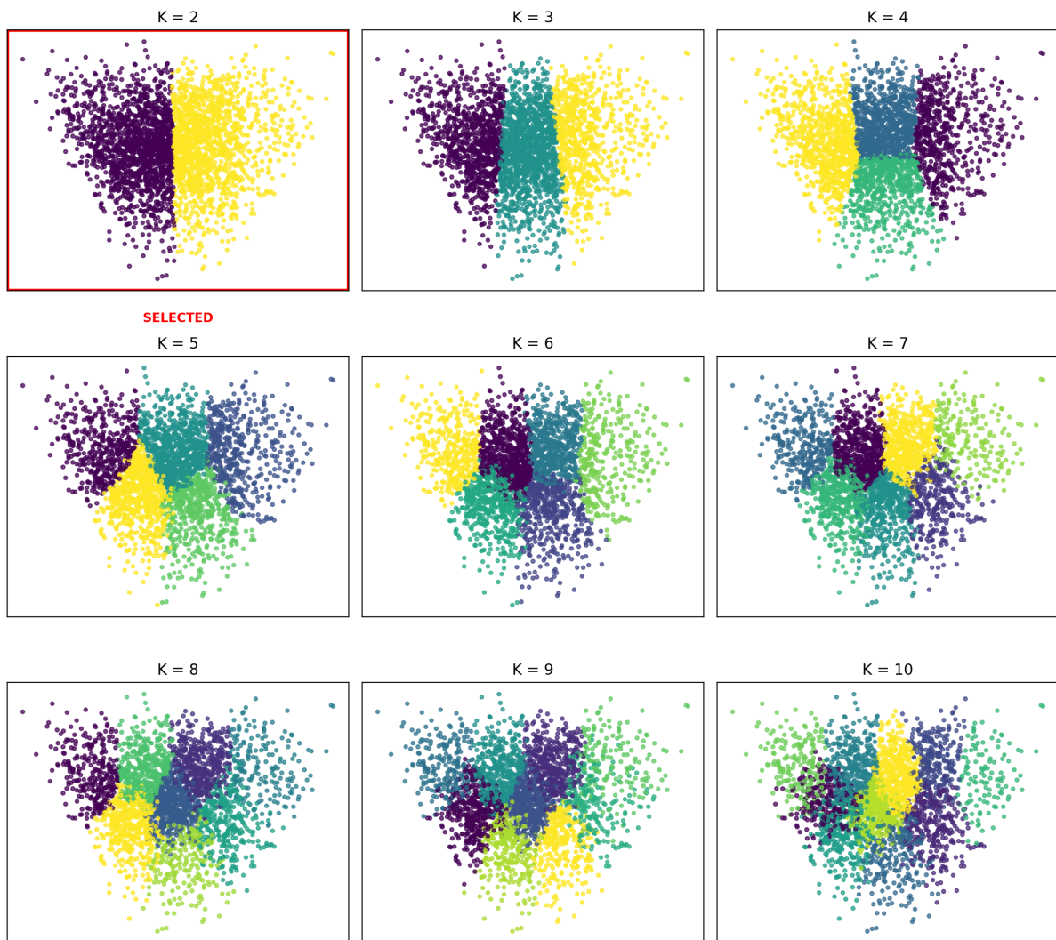
PCA Projection of Lottery Draws (K = 2-10)
