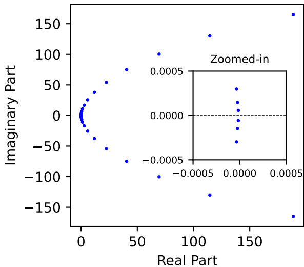
Poles of S(\omega)
