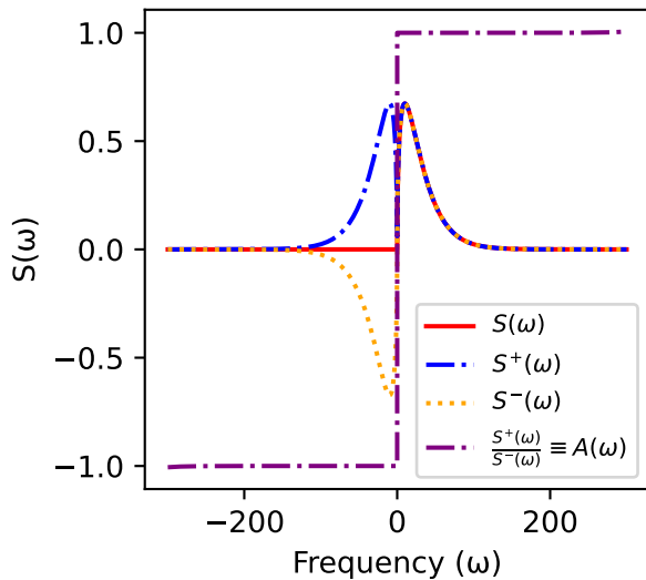
S(\omega) and derived functions
