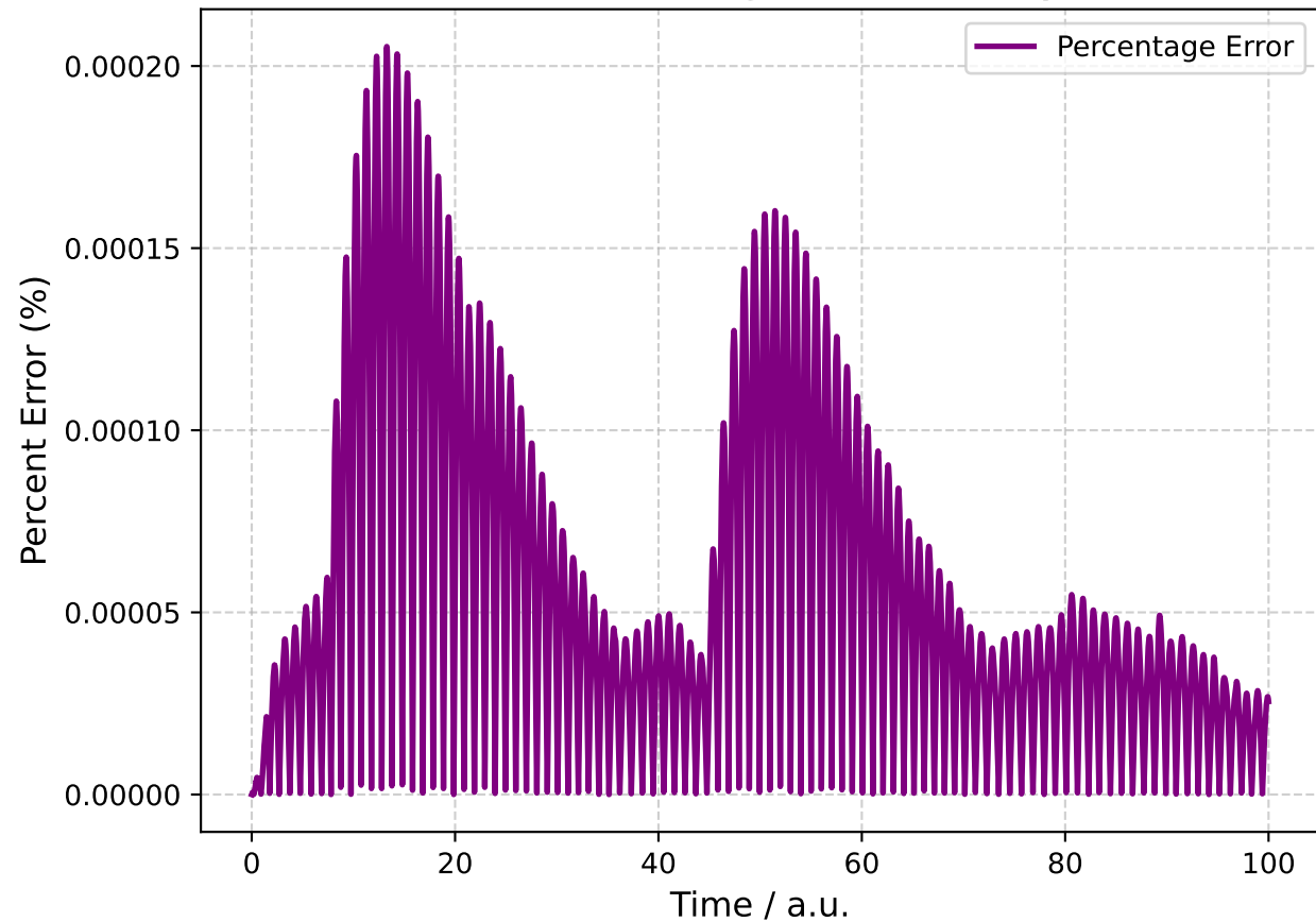
HEOM Convergence Accuracy
