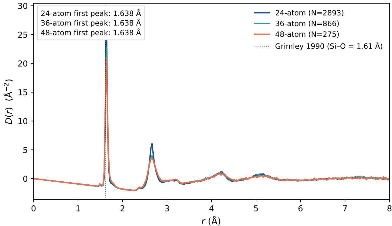
Fig. S1 — Boltzmann-weighted reduced PDF D(r) vs cell size
