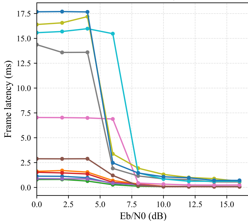
16QAM latency
