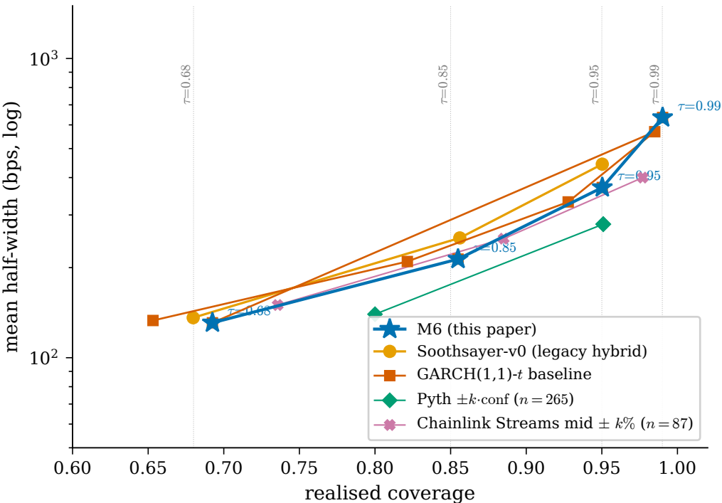
Coverage vs sharpness across methods at four served \tau
