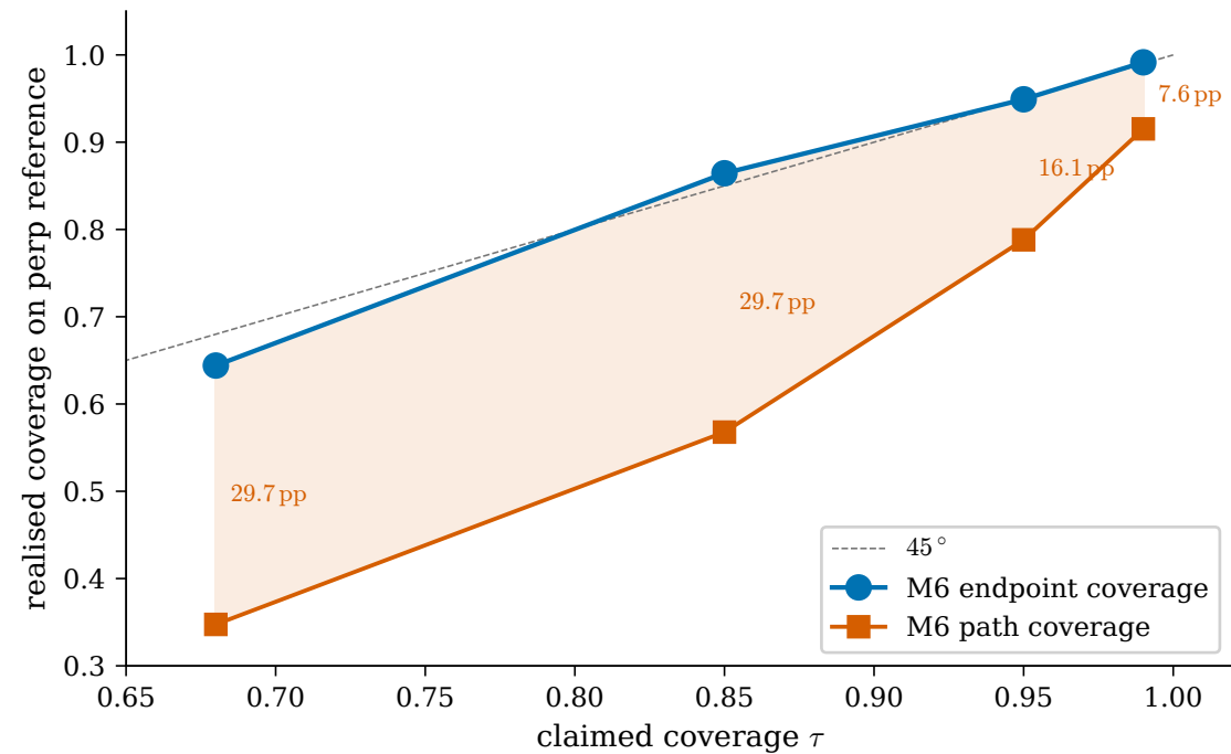
M6 endpoint vs path coverage across \tau ( n = 118 symbol-weekends, 2025-12 \rightarrow 2026-04)
