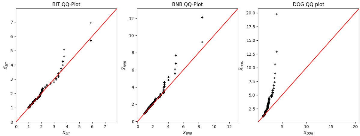
Figure 5: Simulated Returns
