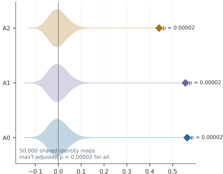
A Frozen controller-label QAP
