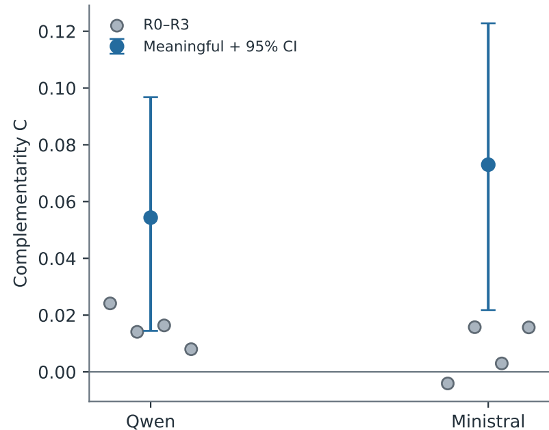
Positive and null-specific C
