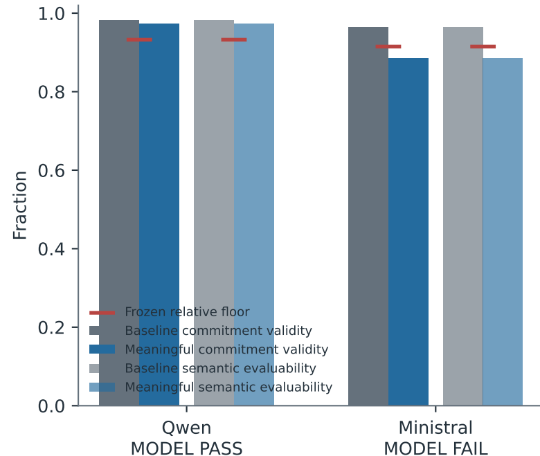
Safe realization is conjunctive
