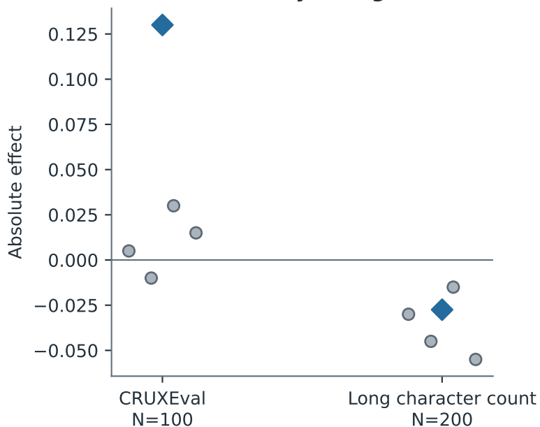
Accuracy change
