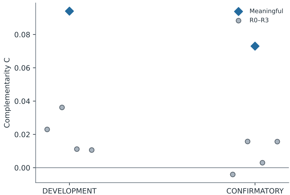
Ministral
