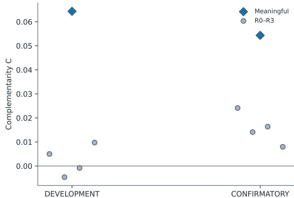
Qwen
