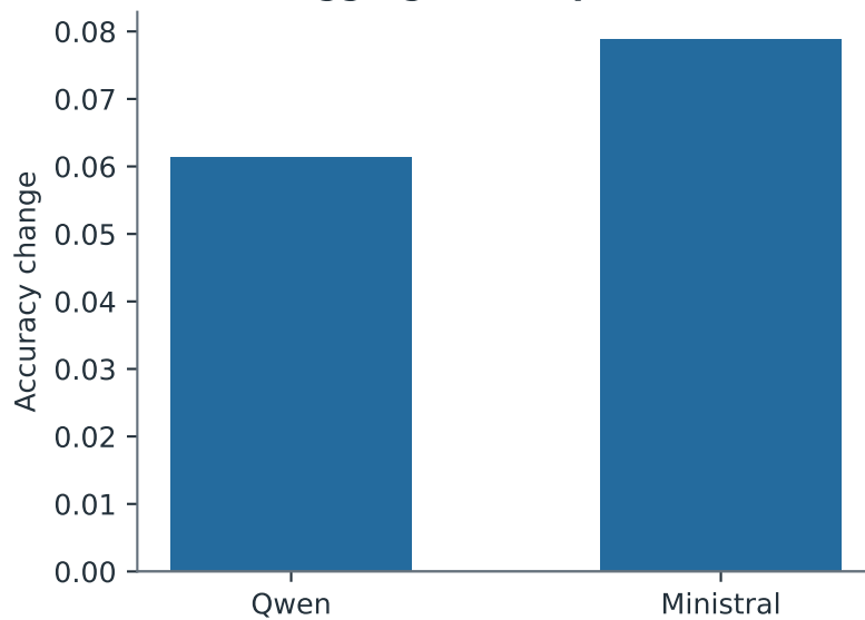
Aggregate competence
