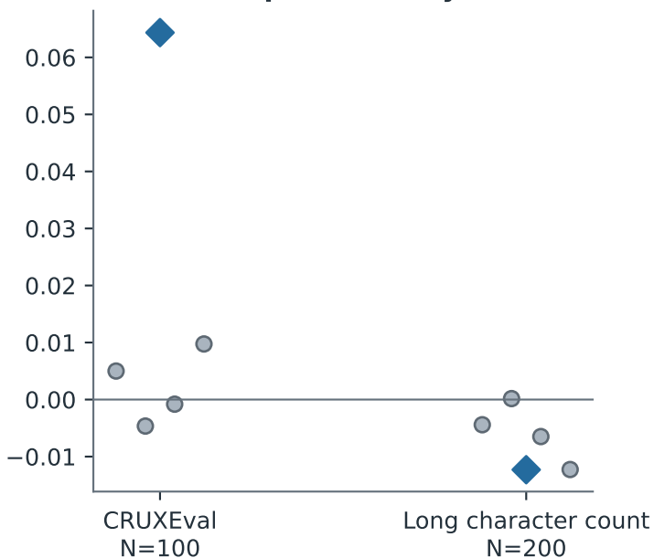
Complementarity C
