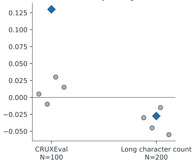
Accuracy change
