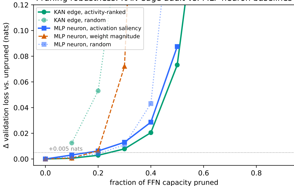
Pruning robustness: KAN edge audit vs. MLP neuron baselines
