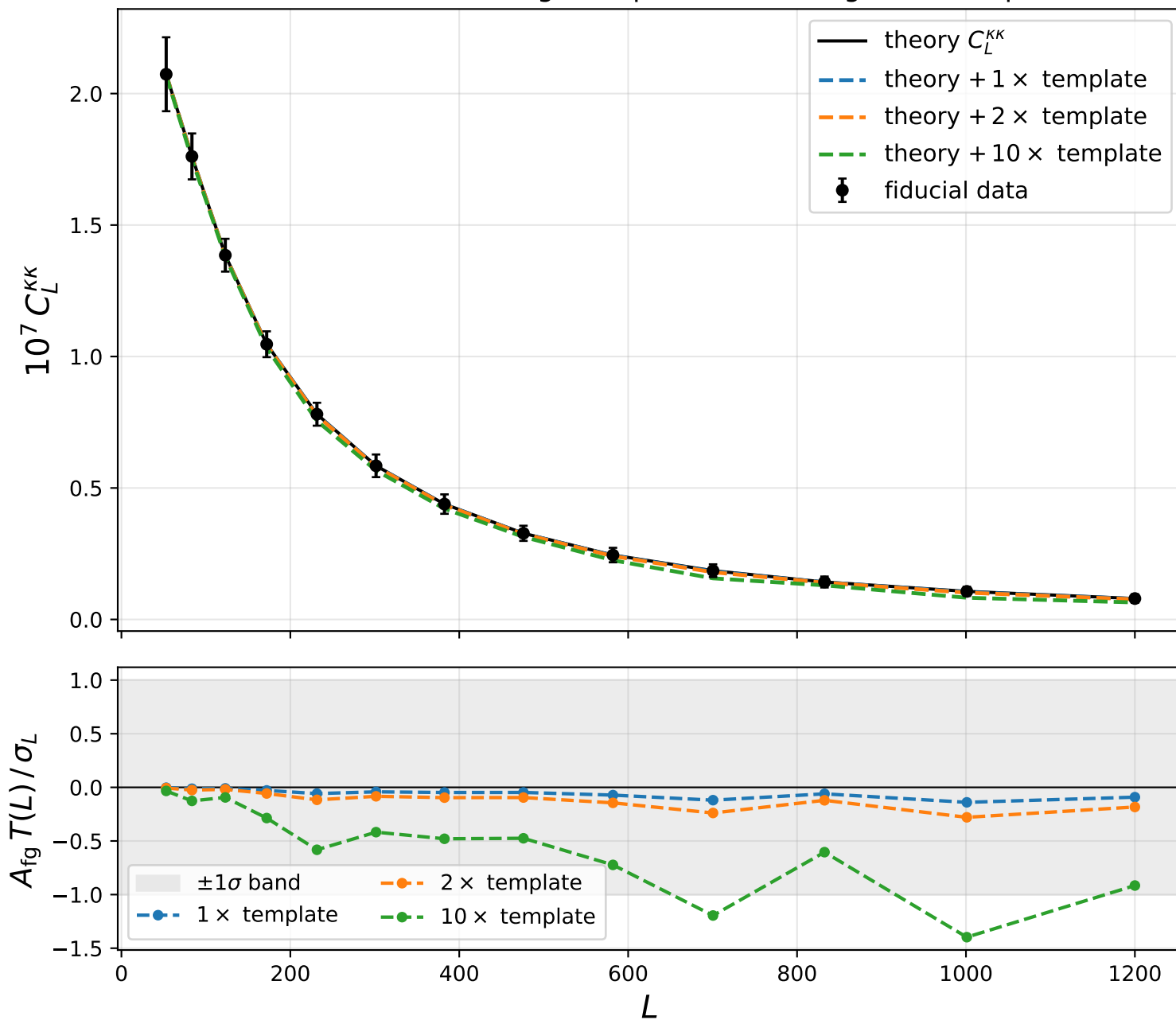
DR6+ extended lensing bandpowers vs. foreground template
