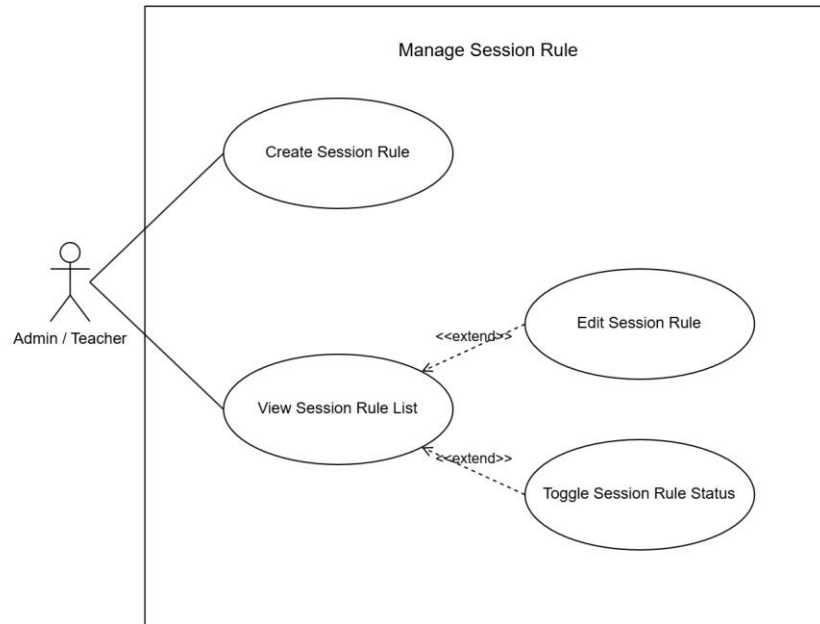
Figure 3.11: System Use Case for Manage Session Rule
