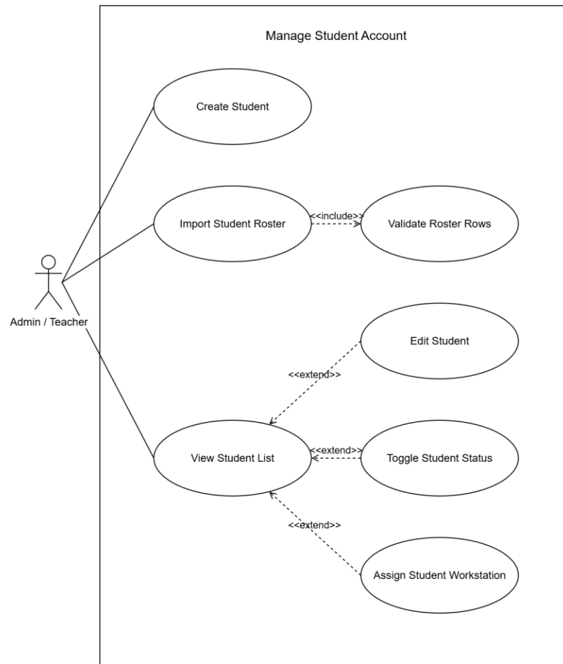
Figure 3.5: System Use Case for Manage Student Account
