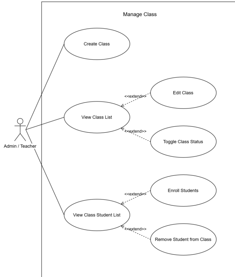
Figure 3.7: System Use Case for Manage Class
