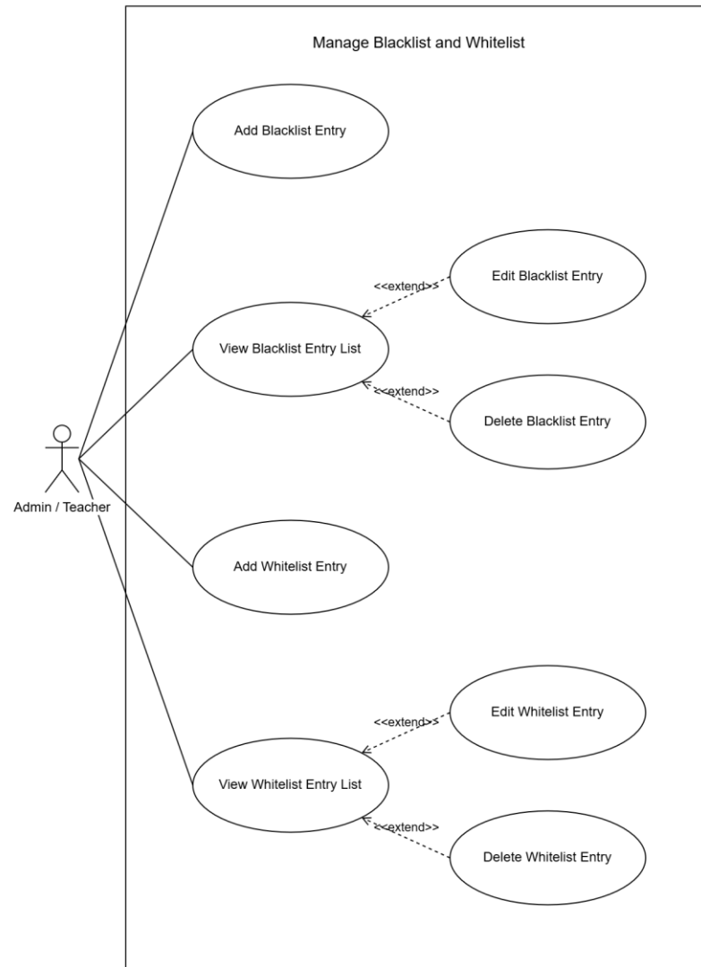
Figure 3.9: System Use Case for Manage Blacklist and Whitelist
