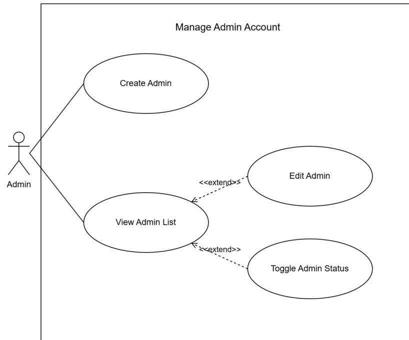
Figure 3.13: System Use Case for Manage Admin Account
