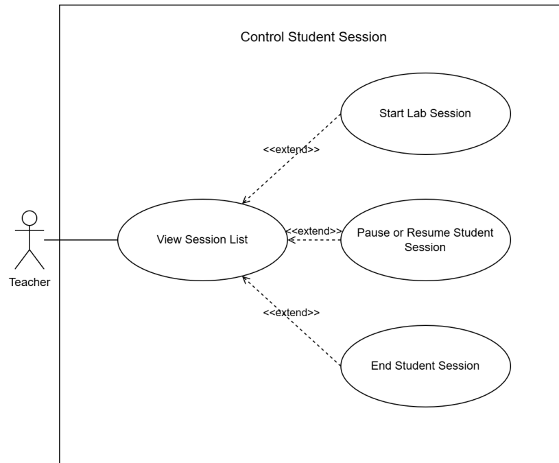
Figure 3.18: System Use Case for Control Student Session
