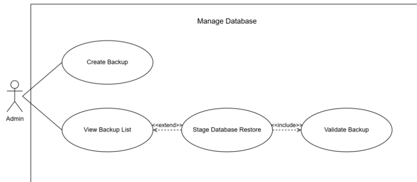
Figure 3.16: System Use Case for Manage Database
