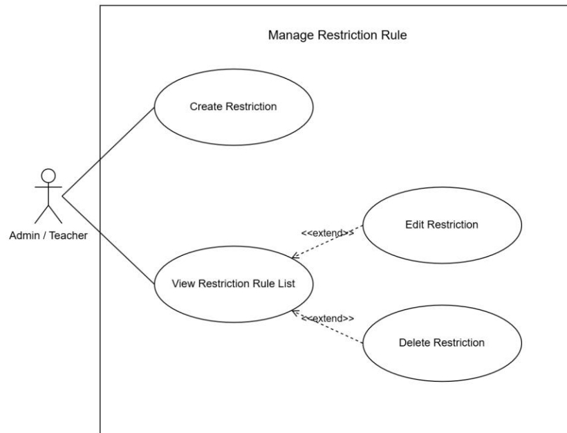
Figure 3.8: System Use Case for Manage Restriction Rule
