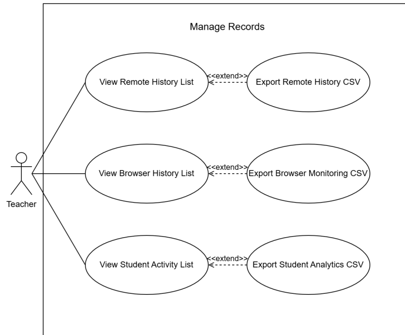
Figure 3.23: System Use Case for Manage Records
