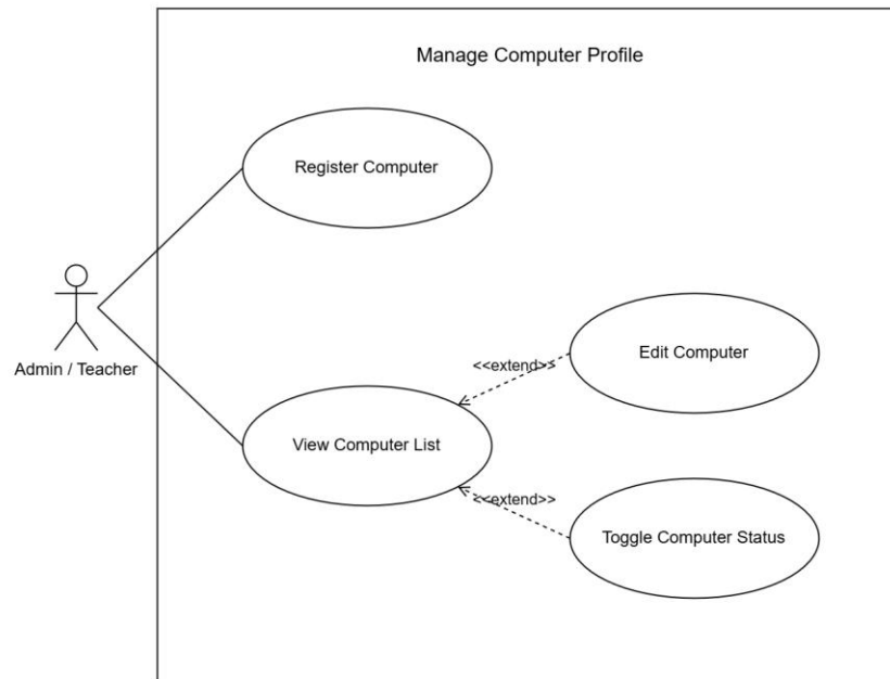
Figure 3.6: System Use Case for Manage Computer Profile
