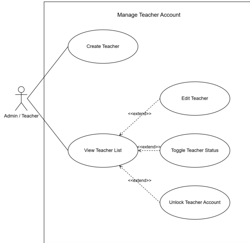
Figure 3.4: System Use Case for Manage Teacher Account
