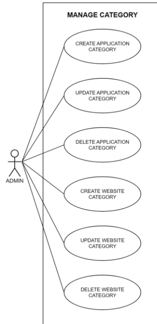
Figure 3.11: System Use Case for Manage Category
