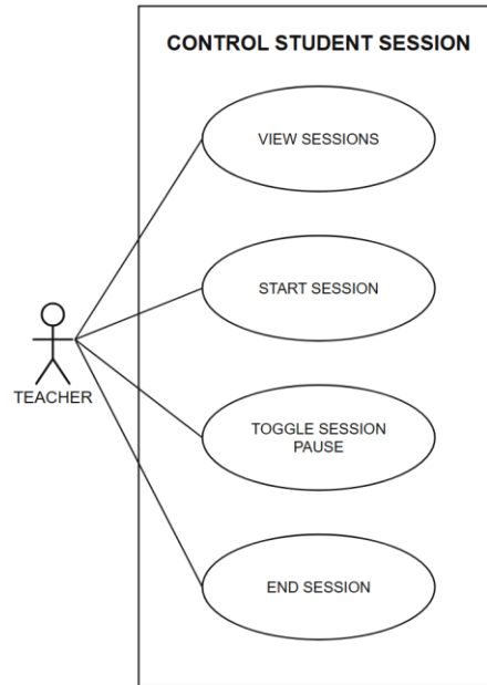
Figure 3.30: System Use Case for Control Student Session
