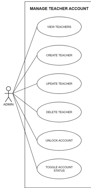
Figure 3.4: System Use Case for Manage Teacher Account
