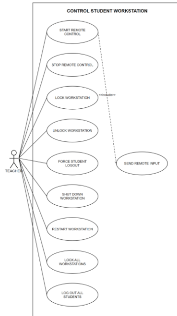
Figure 3.32: System Use Case for Control Student Workstation
