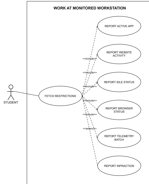
Figure 3.37: System Use Case for Work At Monitored Workstation
