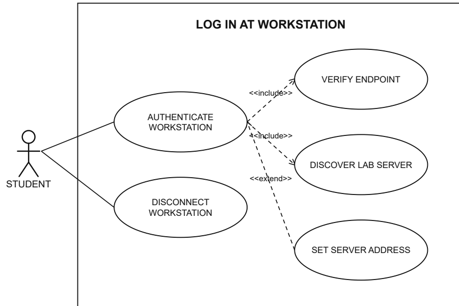
Figure 3.36: System Use Case for Log In At Workstation
