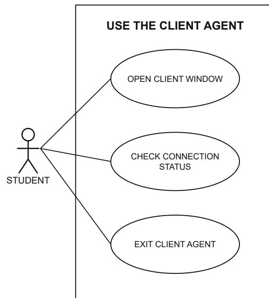
Figure 3.38: System Use Case for Use The Client Agent
