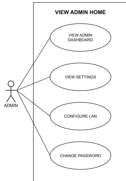
Figure 3.2: System Use Case for View Admin Home
