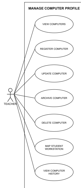
Figure 3.22: System Use Case for Manage Computer Profile
