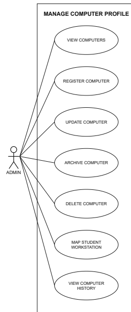
Figure 3.6: System Use Case for Manage Computer Profile
