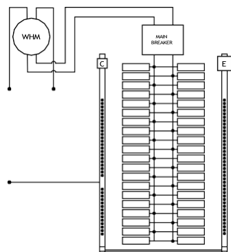
TSM4020UWCU
