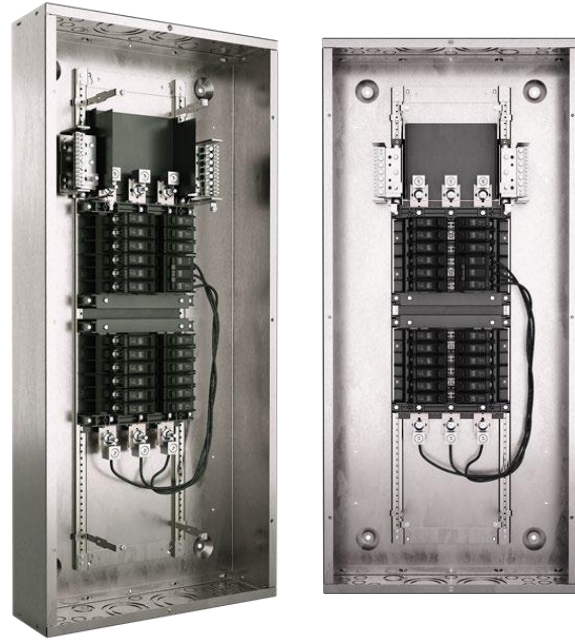
Split Bus
