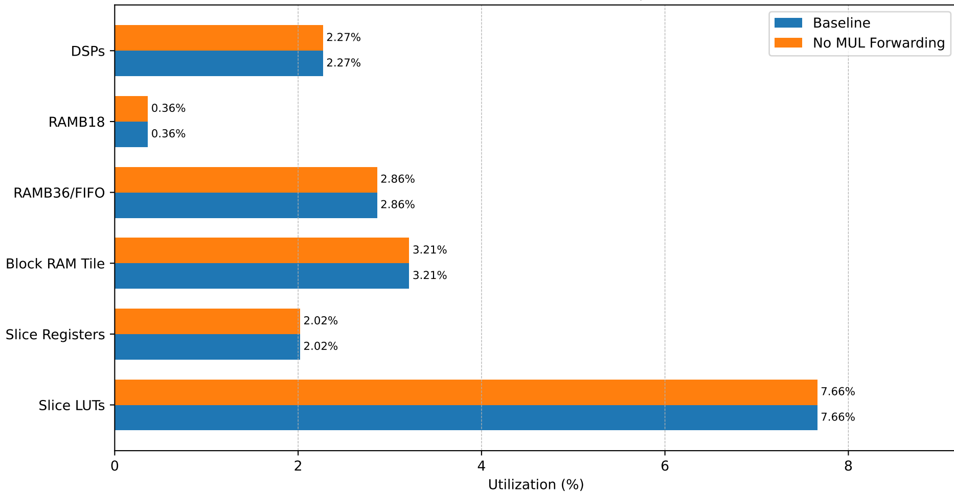
Vivado Resource Utilization Comparison
