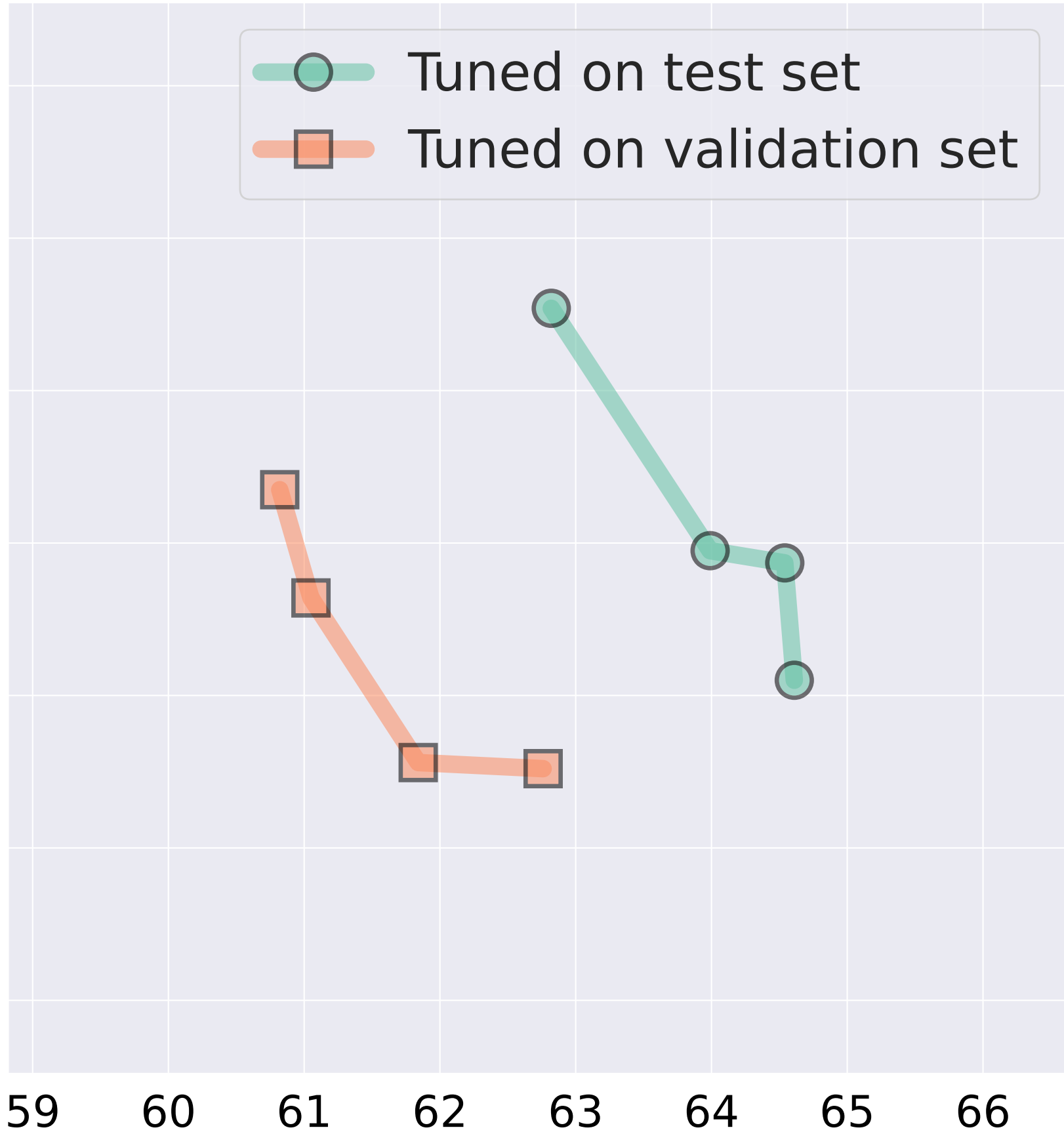
Certified Accuracy
