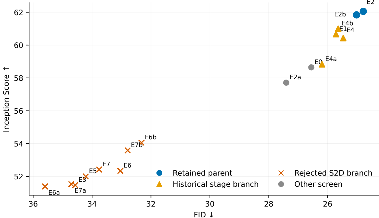
Seed-42 screening: quality frontier and rejected branches
