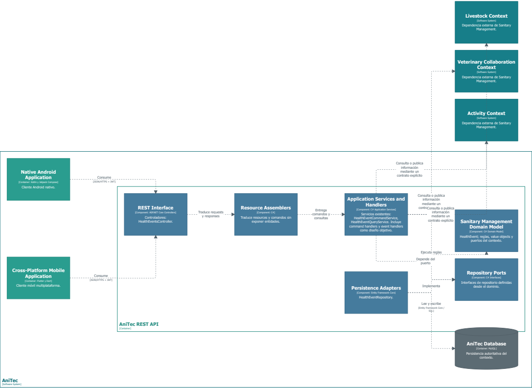
Component View: AniTec - AniTec REST API Componentes backend de Sanitary Management. Tuesday, September 15, 2026 at 3:26 AM Coordinated Universal Time
