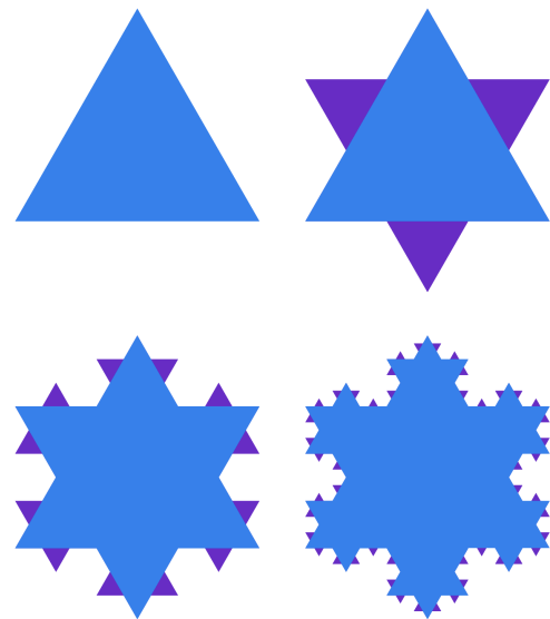
Figure 1.10. Construction of Koch Snowflake [TIF25]
