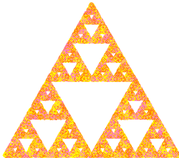
Figure 1.6. Sierpiński Gasket Generated on R
