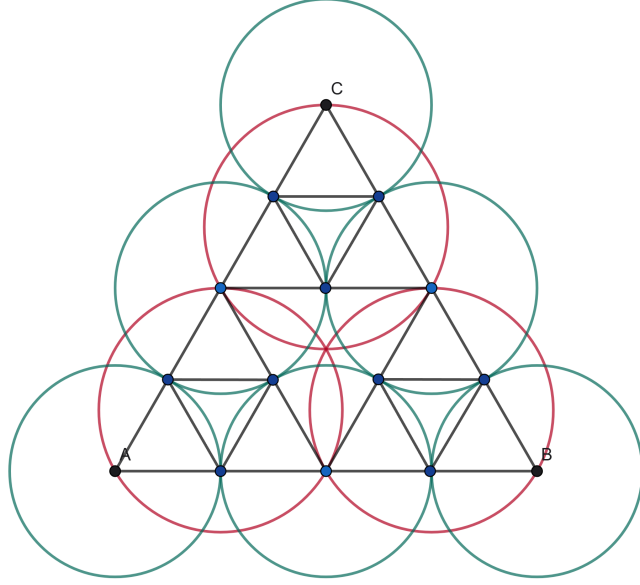
Figure 4.2. Refinement of a Cover of T_1
