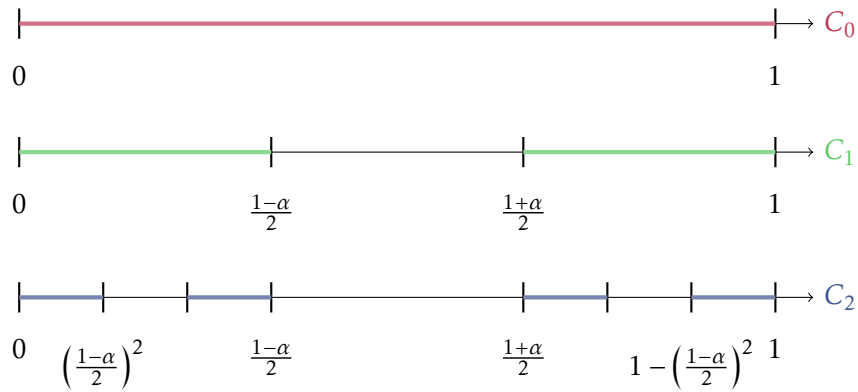
Figure 1.4. The First Three Iterations of C^\alpha
