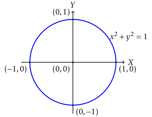
Figure 1.3. Circle S^1 \subset \mathbb{R}^2
