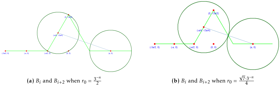
Figure 4.4. B_i and B_{i+2} where a = 3^{-n}
