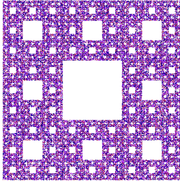
Figure 1.8. Sierpiński Carpet Generated on R
