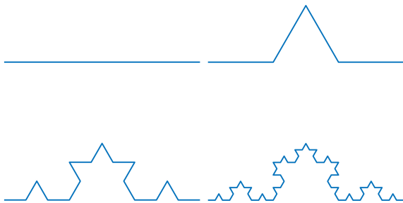
Figure 1.9. Construction of the Koch Curve [TIF25]
