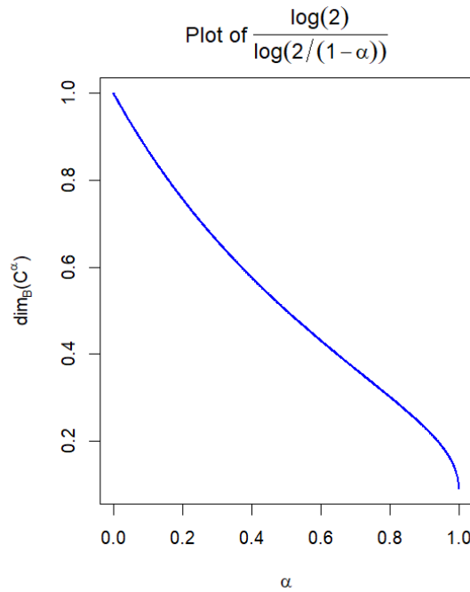
Figure 4.1. Plot of \alpha vs \dim_B(C^\alpha)
