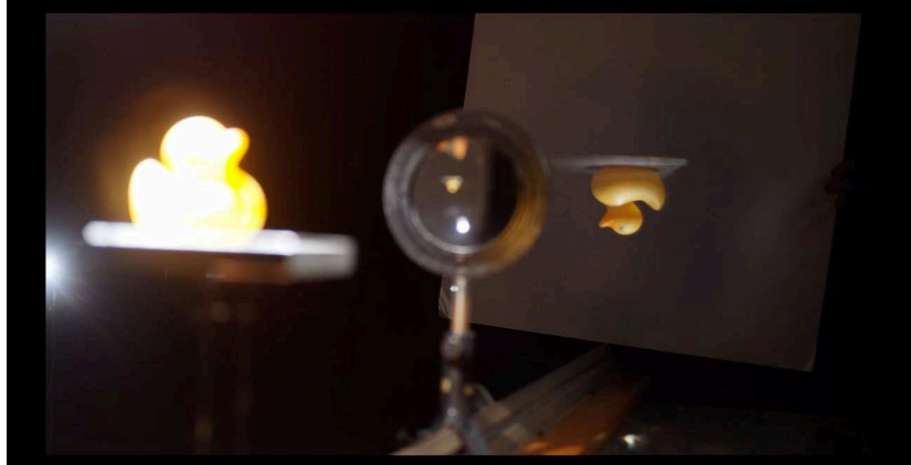
Figure 136: Real image formation by a converging lens. A brightly illuminated rubber duck (left) serves as the object for a convex (converging) lens positioned at center. The lens refracts diverging rays from the duck and brings them to a focus on a screen at right, forming a real, inverted image.
