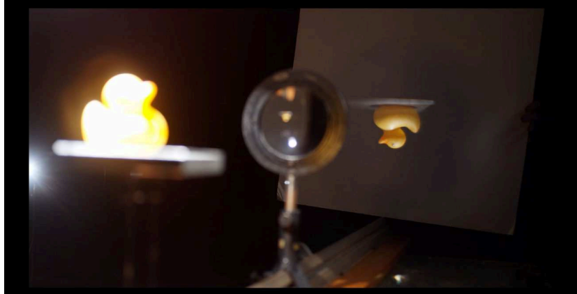
Figure 136: Real image formation by a converging lens. A brightly illuminated rubber duck (left) serves as the object for a convex (converging) lens positioned at center. The lens refracts diverging rays from the duck and brings them to a focus on a screen at right, forming a real, inverted image.
