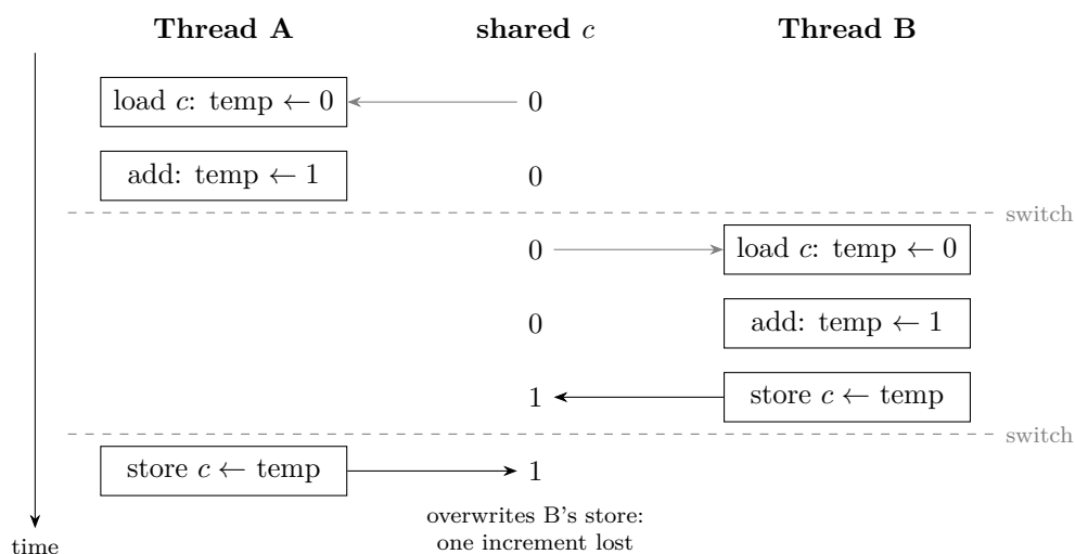
Figure 31: The lost update of Example 19.74. Time runs downward; the middle column shows the shared value after each step. Thread A loads 0 and computes 1, the scheduler switches (dashed line) at the first hand-off, thread B loads the same 0, computes 1 and stores it, and after the second hand-off thread A stores its stale 1 over B ’s. Two increments, final value 1. Nothing in the picture depends on the GIL: the two switches are the hand-offs Fact 19.73 permits.
