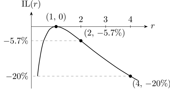
Figure 25: Impermanent loss IL(r) = 2\sqrt{r}/(1+r) - 1 of (15.2) against the gross price ratio r . The curve touches zero only at r = 1 and is negative in both directions — the left branch shows that a sell-off hurts the LP too. Marked points: (1, 0) , (2, -5.7\%) , (4, -20\%) .
