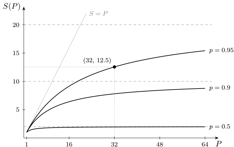
Figure 29: Amdahl speedup (19.2) against the processor count for p = 0.5 , 0.9 and 0.95 , with the ceilings 1/(1 - p) = 2 , 10 and 20 as dashed lines and the ideal S = P in light gray. The marked point is S(32) = 12.5 at p = 0.95 (Example 19.38); doubling to 64 processors reaches only 15.4.
