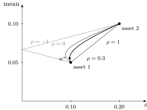
Figure 18: Long-only mixes of the two assets of Example 11.5 (volatilities 10% and 20%, means 5% and 10%) in the (\sigma, \text{mean}) plane. At \rho = 1 the mixes lie on the straight segment joining the assets; at \rho = 0.3 (black) and \rho = 0 (gray) they trace curves bulging leftward, and the curves nest leftward as \rho falls; at \rho = -1 they form a V touching the vertical axis at mean 6.67%. The leftmost point of each curve is the minimum-variance mix of Proposition 11.4(ii) — marked w^* at (9.79%, 5.53%) for \rho = 0.3 — and the \rho = \pm 1 curves are the straight lines of part (iv). With two assets every fully invested portfolio lies on its curve, so each curve is also the n = 2 version of the frontier of Figure 19.
