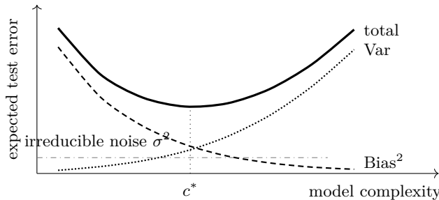
Figure 13: The bias–variance trade-off of Theorem 8.2 as model complexity grows: squared bias falls (dashed), variance rises (dotted), the irreducible noise \sigma^2 is a constant floor (dash-dotted), and their sum — the expected test error (solid) — is U-shaped, minimized at an interior complexity c^* .
