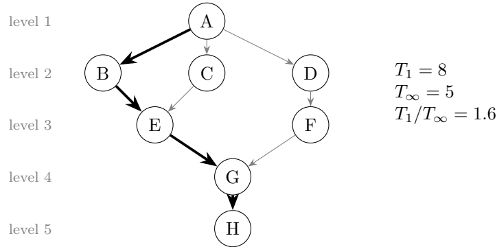
Figure 30: The eight-task DAG of Example 19.17, scheduled in Example 19.42: a critical path, A–B–E–G–H (thick), has length T_\infty = 5 — one of three of that length, the other two running through C and through D–F — and the remaining edges are gray. The levels are the earliest steps at which tasks can run, which are Kahn’s waves. With three processors the greedy schedule finishes in 5 steps, so the span law of Theorem 19.41(i) is tight and a fourth processor buys nothing.
