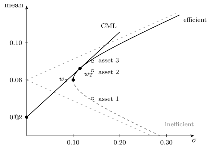
Figure 19: The mean–variance frontier of the running universe (Example 11.17) in the (\sigma, \text{mean}) plane. The vertex w_g = (0.5, 0, 0.5)^\top at (10\%, 6\%) is Theorem 11.7; the curve \sigma^2 = 0.01 + 20(m - 0.06)^2 is Theorem 11.16 and Corollary 11.18, with its asymptotes of slope \pm 0.2236 dashed in gray; the upper branch is efficient, the lower (dashed) branch is dominated. The three assets stack vertically at volatility 14.14% because all three volatilities are equal, and lie strictly inside the hyperbola. The straight line from r_f = 2\% on the vertical axis is the capital market line (11.12) of Corollary 11.27 in §11.4; it lies weakly above the hyperbola everywhere and touches it only at the tangency portfolio w_T at (11.46\%, 7.25\%) .
