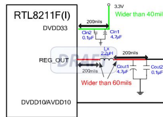
Figure 10. Switching Regulator
