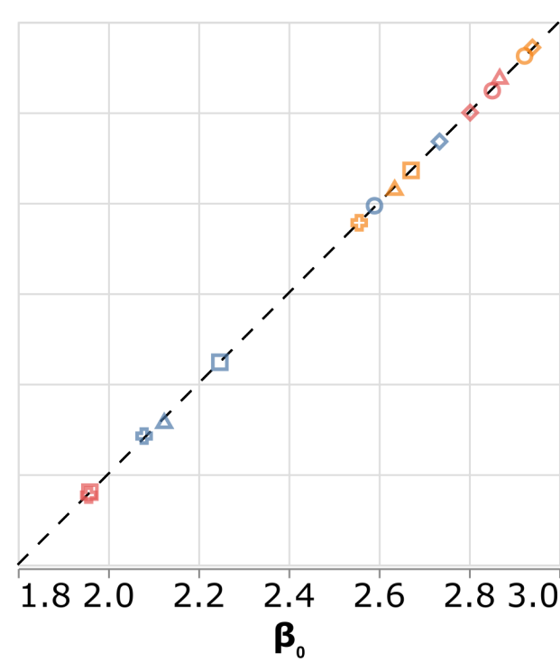
MC (N = 1000)
