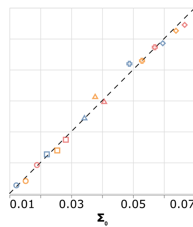
MC (N = 1000)
