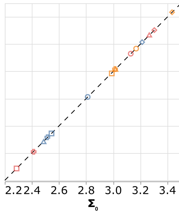
Monte Carlo (N = 100000)
