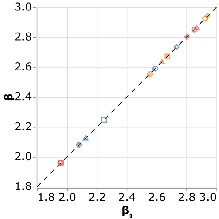
Variance estimation
