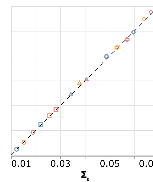
MC (N = 10000)
