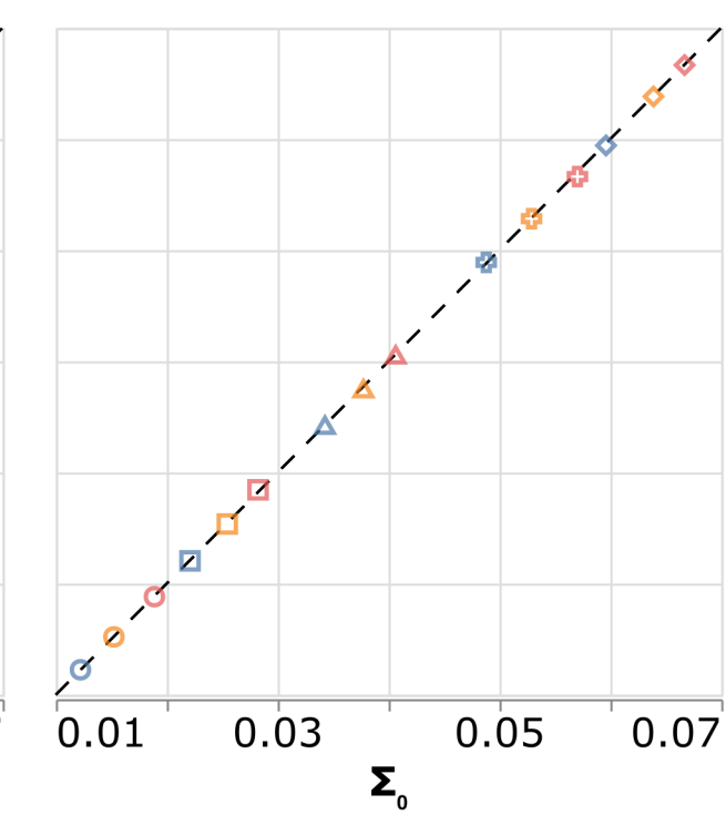
MC (N = 100000)
