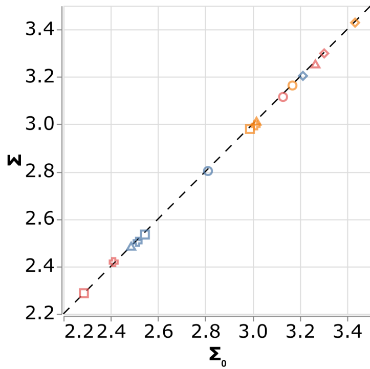
Uncertainty propagation method
