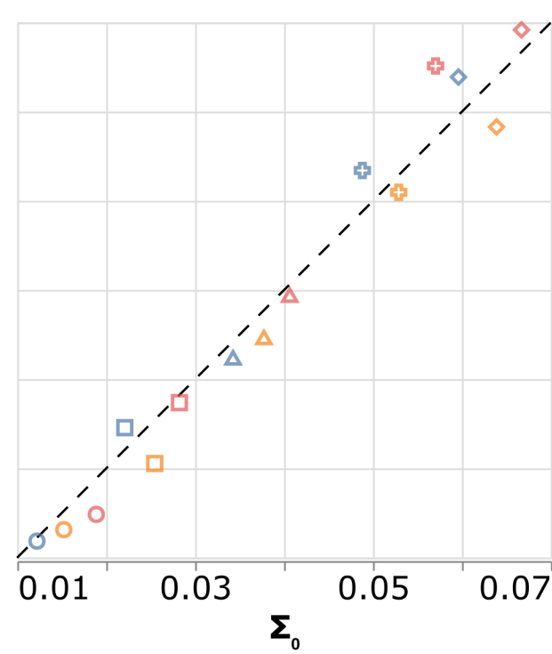
MC (N = 100)
