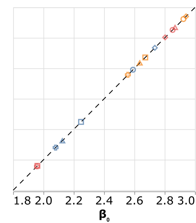
MC (N = 100000)
