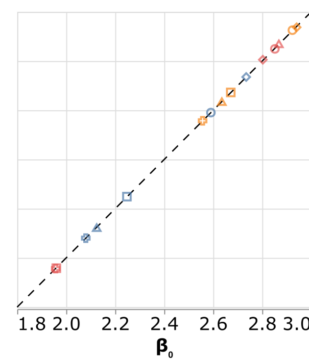
MC (N = 10000)
