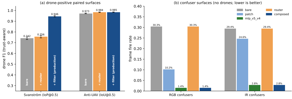
Figure 5.1: Pipeline ablation at a glance for the shipped robust8-nr cascade (filter-then-route composition). (a) Drone-positive paired surfaces: the always-routing router adds a small per-modality lift and the per-frame filter finishes it (Svanström 0.742 \rightarrow 0.946); Anti-UAV confirms no-harm. Whiskers are 95% bootstrap confidence intervals (the central range of the metric over 1,000 resamples of the frames; bars whose whiskers do not overlap differ by more than sampling noise). (b) Confuser surfaces: bare \rightarrow patch \rightarrow mlp_v5_v4 \rightarrow router \rightarrow composed frame fire rates. The no-reject router never vetoes a confuser frame, so its router-only bar stays at the bare rate and the per-frame filter owns suppression: RGB 30.4% \rightarrow 1.4% composed, thermal 29.4% \rightarrow 2.8%. Generated from results_noreject/tier1_results.json by thesis_eval/gen_ablation_figure.py .
