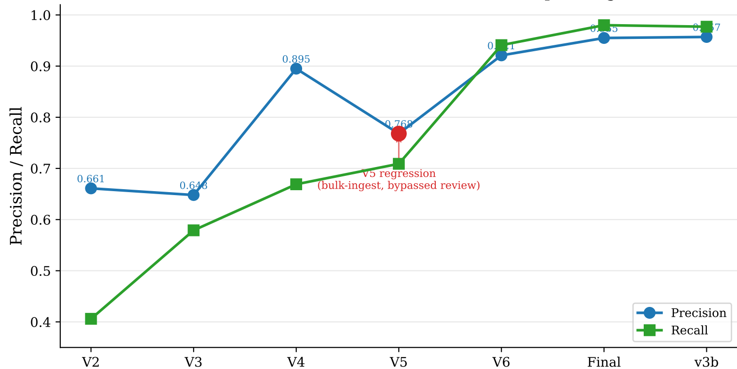
IR detector P/R across HITL revisions (fixed test split, imgsiz=640)
