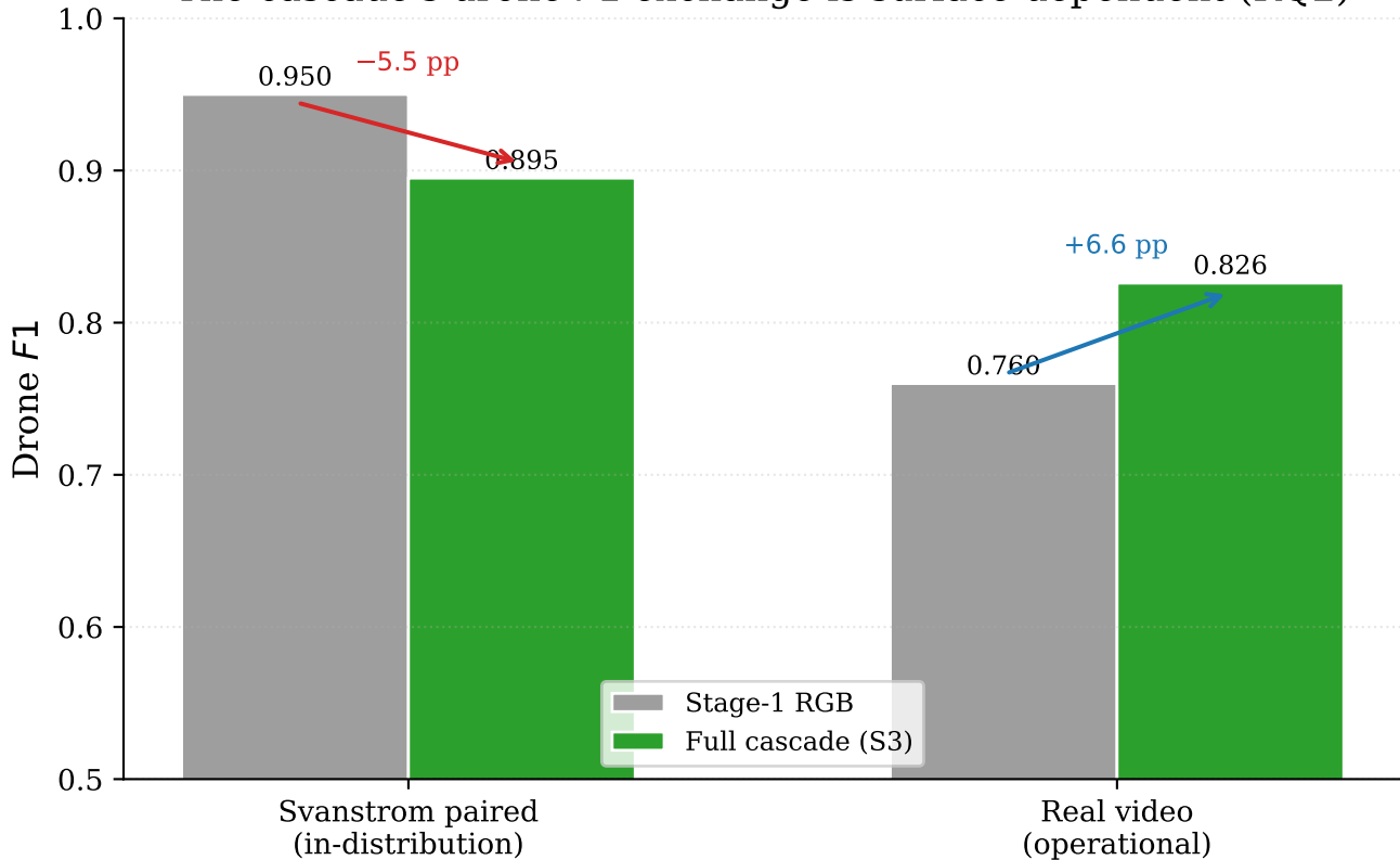
The cascade's drone- F1 exchange is surface-dependent (RQ2)
