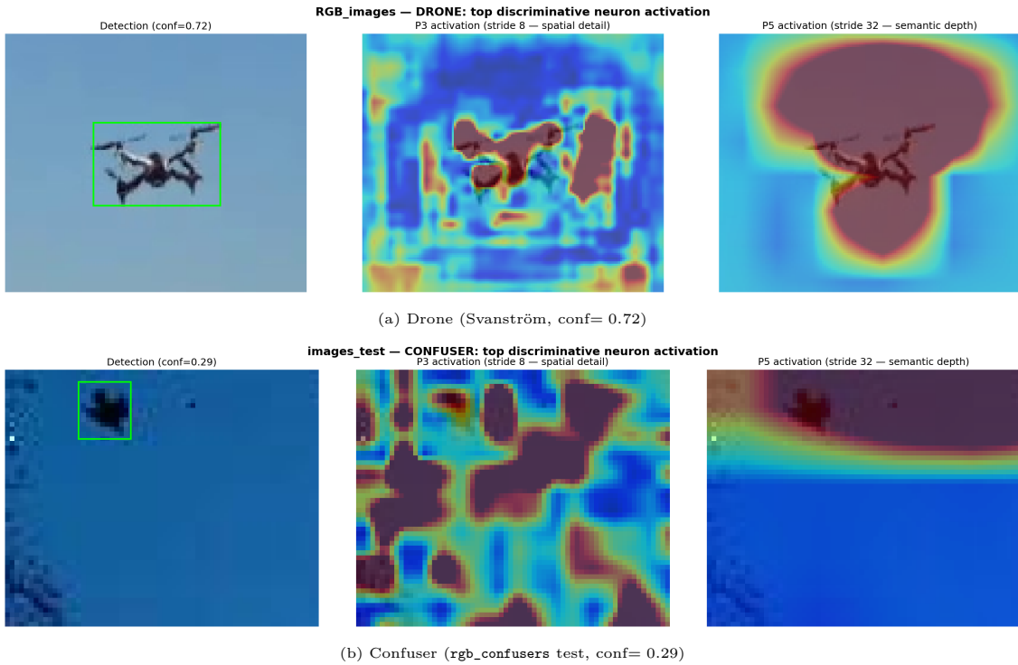
Figure 5.4: Model MRI spatial “brain scan” of the top discriminative neurons. Each row: the detection crop, the p3 activation (stride 8, fine spatial detail), and the p5 activation (stride 32, semantic depth). On the drone (a) p3 binds to the airframe and p5 forms a centred semantic blob; on the confuser (b) the same neurons fire diffusely across background structure. This activation-signature difference is what the feature-reuse filter reads.
