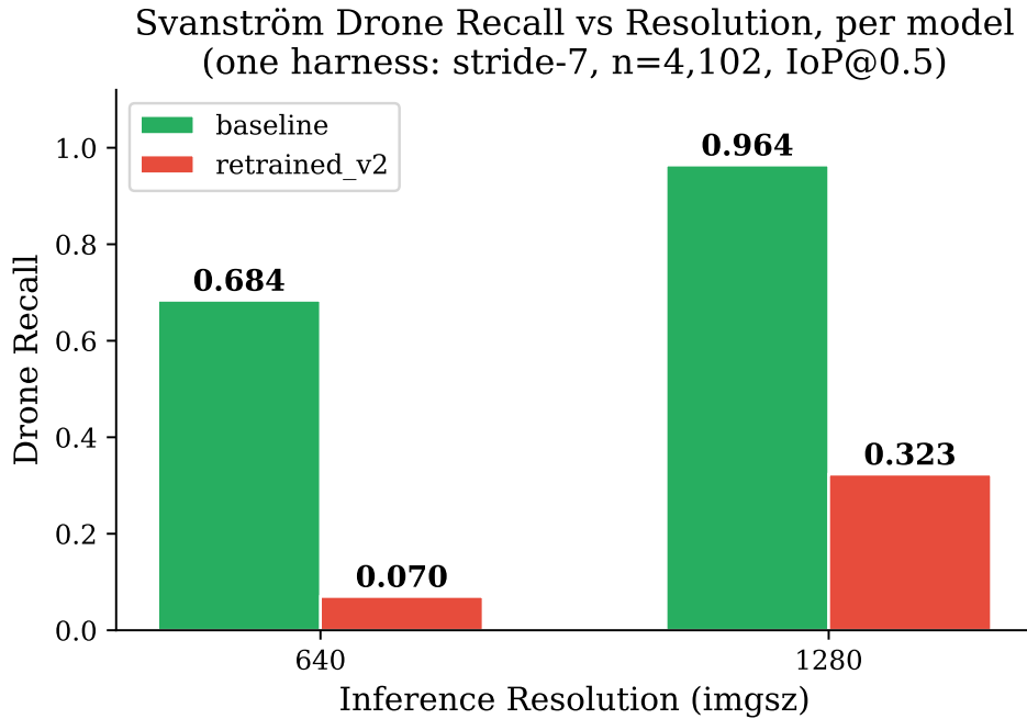
Figure 3.4: Inference-resolution dependency of Svanström drone recall, isolated within each model (one harness: stride-7 sample, n = 4,102 , IoP@0.5, conf 0.25). Doubling imgsz buys both variants a similar recall increment ( +28 pp baseline, +25 pp retrained_v2 ); the absolute level is set by the training stance. The confuser-suppressing retrained_v2 is unusable on Svanström at either size.
