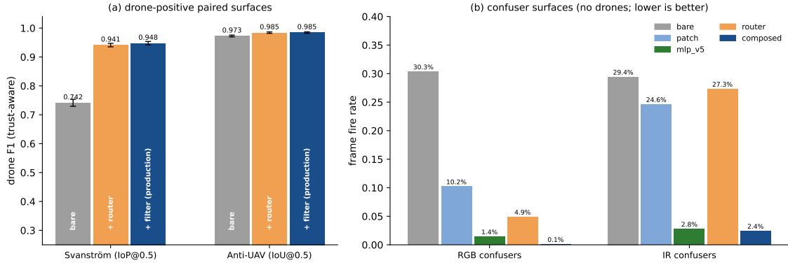
Figure 5.5: Pipeline ablation at a glance, drawn for the reject-class robust8 cascade (the strongest-suppression configuration; the shipped no-reject robust8-nr trades part of the confuser suppression for recall, Table G.4). (a) Drone-positive paired surfaces: the router supplies most of the F1 lift and the filter finishes it; Anti-UAV confirms no-harm. Whiskers are 95% bootstrap confidence intervals (the central range of the metric over 1,000 resamples of the frames; bars whose whiskers do not overlap differ by more than sampling noise). (b) Confuser surfaces: bare \rightarrow patch \rightarrow mlp_v5 \rightarrow router \rightarrow composed frame fire rates, with near-total suppression on RGB (30.4% \rightarrow 0.11% composed) and thermal-confuser fire now largely suppressed by the thermal-native filter (29.4% \rightarrow 2.4% composed); the shipped no-reject stack delegates suppression to the filter alone and sits at 1.4% on RGB.
