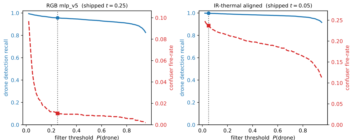
Figure 5.2: Filter operating points (detection level). For each production confuser filter, drone detection recall (blue, left axis; fraction of GT-matched true-drone detections retained, pooled over the drone surfaces) and confuser fire-rate (red dashed, right axis; matching confuser surface) as the per-detection P(\text{drone}) threshold varies; the shipped point ( t = 0.25 RGB, 0.05 IR-thermal) is marked. RGB sits on a flat high-recall shoulder; the thermal-native head now suppresses thermal confusers (fire falls with the threshold; the residual is the airplane-like in-distribution fraction). Source: eval/filter_operating_sweep.py .
