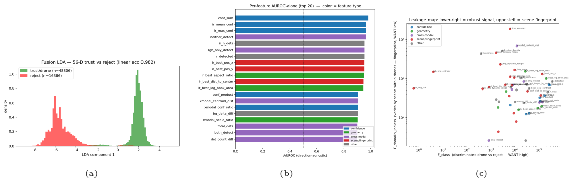
Figure 3.5: Statistical anatomy of the 56-feature fusion space. (a) Linear discriminant: the trust signal is linearly separable (98.2% train accuracy). (b) Per-feature single-feature AUROC. (c) Leakage map (Eq. 3.1): the lower-right region is robust signal (high AUROC, near-zero leakage); the upper-left is scene fingerprint (chance-level AUROC, leakage in the hundreds). Source: classifier/fusion_feature_stats.py .
