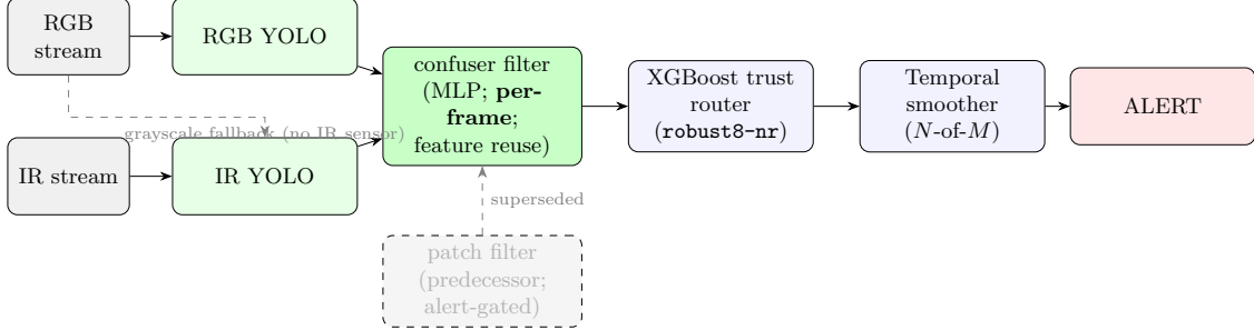
Figure 3.1: Multi-stage drone detection pipeline in the production composition: detectors, then the confuser filter, then the trust classifier. The order itself was ablated (Section 5.3): filter-first ships because it edges classifier-first on Svanström ( F1 = 0.946 vs 0.931 ), and the two are within about a point on the paired benchmarks. The production confuser filter is the distilled mlp_v5_v4 (RGB) with its paired thermal-native IR head, which runs per frame because it reuses the detectors’ already-computed internal features rather than re-processing crops (Section 3.11). It supersedes the MobileNetV3 patch filter (greyed), which was expensive enough that it had to be alert-gated : consulted only when the temporal smoother was about to fire (Section 3.4).
