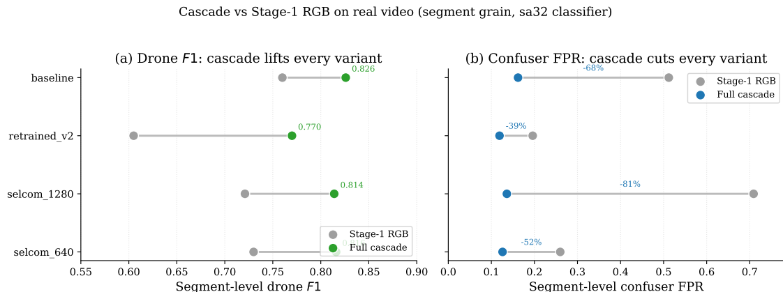
Figure 5.6: Design-evolution record (predecessor stack: baseline RGB, sa32, alert-gated patch): segment-level drone F1 and confuser FPR, Stage-1 RGB (grey) versus the full cascade, on the real-video diagnostic. (a) The cascade lifts drone F1 for every variant. (b) It cuts confuser FPR by 39–81%. The production-stack re-run of this surface is Table 5.11.
