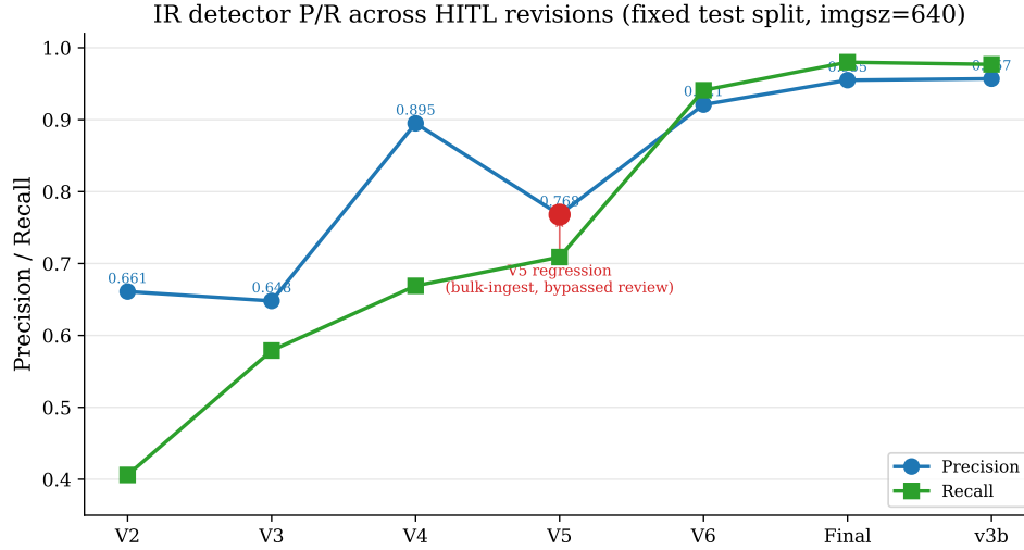
Figure 5.1: IR detector P/R trajectory across the five numbered revisions (V2–V6) plus the Final retrain and production v3b , on the fixed IR_dset_final test split. The V5 regression (precision 0.895 \rightarrow 0.768) is recovered by V6 and the production v3b .
