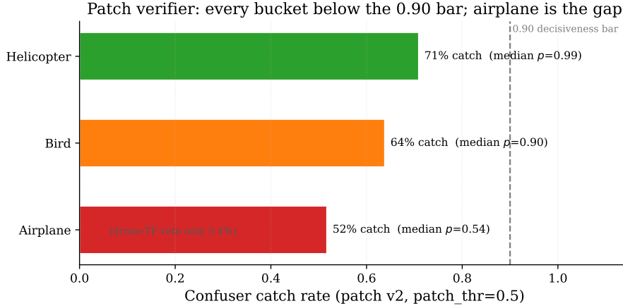
Figure 4.2: Patch-filter (v2) per-bucket confuser catch rate at patch_thr=0.5 , against the 0.90 “decisiveness” bar. Helicopters (71%) and birds (64%) are mid; airplanes (52%, median patch probability 0.540) are the actionable gap. All three buckets sit below the bar, the motivation for the feature-reuse successor.
