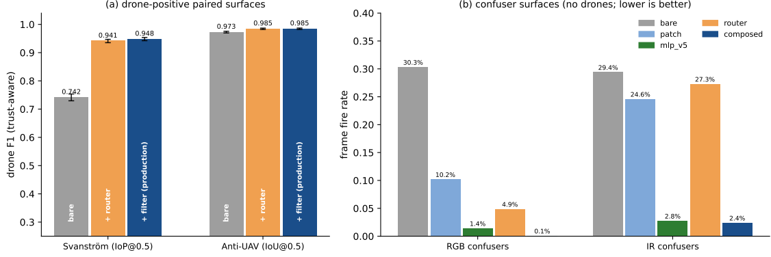
Figure 4.9: Pipeline ablation at a glance, drawn for the reject-class robust8 cascade (the strongest-suppression configuration; the shipped no-reject robust8-nr trades part of the confuser suppression for recall, Table 4.11). (a) Drone-positive paired surfaces: the router supplies most of the F1 lift and the filter finishes it; Anti-UAV confirms no-harm. Whiskers are 95% bootstrap confidence intervals (the central range of the metric over 1,000 resamples of the frames; bars whose whiskers do not overlap differ by more than sampling noise). (b) Confuser surfaces: bare \rightarrow patch \rightarrow mlp_v5 \rightarrow router \rightarrow composed frame fire rates, with near-total suppression on RGB (30.4% \rightarrow 0.11% composed) and thermal-confuser fire now largely suppressed by the thermal-native filter (29.4% \rightarrow 2.4% composed); the shipped no-reject stack delegates suppression to the filter alone and sits at 1.4% on RGB. Generated from tier1_results.json by thesis_eval/gen_ablation_figure.py .
