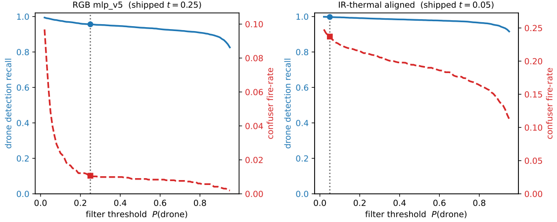
Figure 4.4: Filter operating points (detection level). For each production confuser filter, drone detection recall (blue, left axis; fraction of GT-matched true-drone detections retained, pooled over the drone surfaces) and confuser fire-rate (red dashed, right axis; matching confuser surface) as the per-detection P(\text{drone}) threshold varies; the shipped point ( t = 0.25 RGB, 0.05 IR-thermal) is marked. RGB sits on a flat high-recall shoulder; the thermal-native head now suppresses thermal confusers (fire falls with the threshold; the residual is the airplane-like in-distribution fraction). Source: eval/filter_operating_sweep.py .
