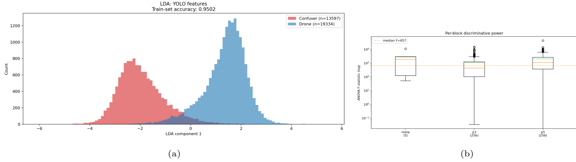
Figure 4.7: Model MRI of the FT4 detector’s fused p3+p5 features on the shipped 32,931-detection corpus. (a) The linear-discriminant projection separates drone (blue) from confuser (red) into two cleanly-resolved peaks at \approx 95\% single-threshold accuracy. (b) Per-block ANOVA F -statistic: p5 is the dominant discriminative layer (max F = 42,346 , median 657), ahead of p3 and the detection metadata; the confidence scalar ranks only 6th.
