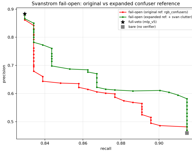
Figure 4.3: Design-history: the recall/precision frontier on Svanström for the no-retrain fail-open gate (with the original rgb_confusers reference, red, versus a reference expanded with held-out Svanström clutter, green), against the full-veto operating point (star) and the bare detector (square). This gate was the candidate fix before the bird-split re-mine closed the coverage gap directly; it is retained only as the record of why a calibration patch was inferior to fixing the training coverage. Source: eval/failopen_expanded_ref.py .
