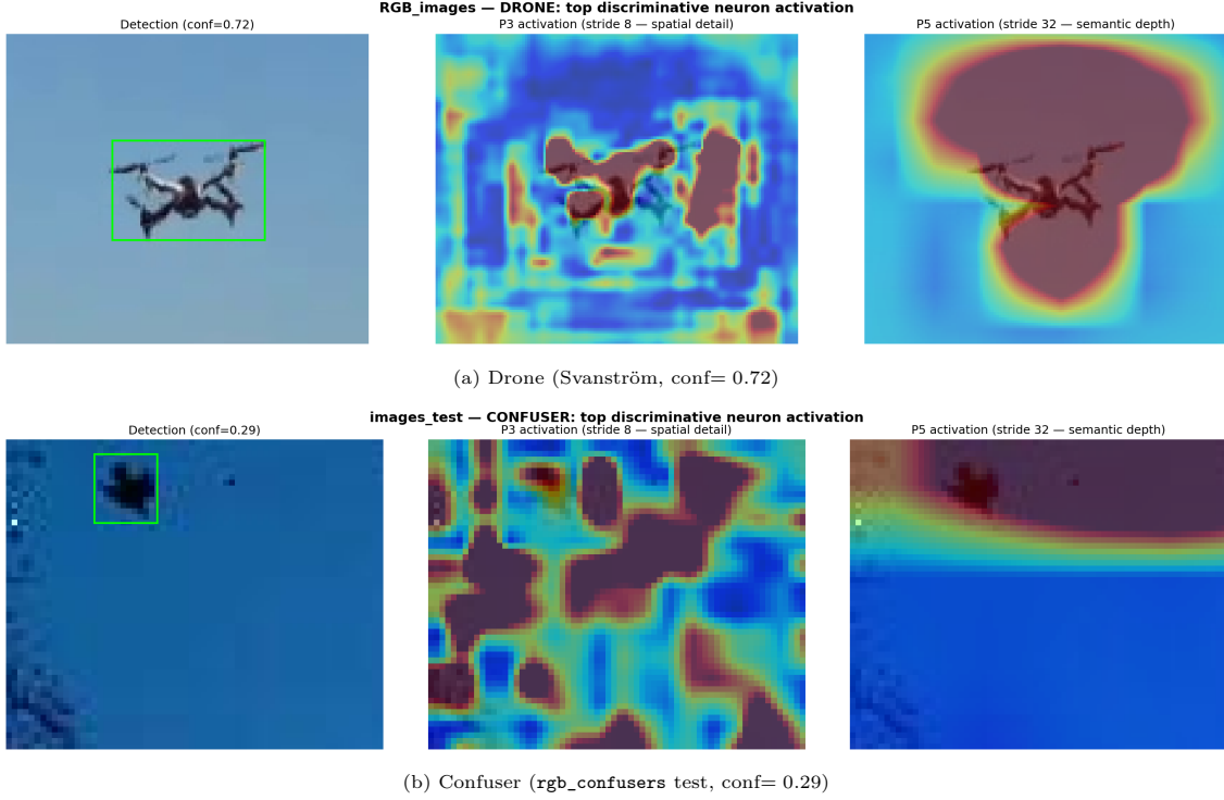
Figure 4.8: Model MRI spatial “brain scan” of the top discriminative neurons. Each row: the detection crop, the p3 activation (stride 8, fine spatial detail), and the p5 activation (stride 32, semantic depth). On the drone (a) p3 binds to the airframe and p5 forms a centred semantic blob; on the confuser (b) the same neurons fire diffusely across background structure. This activation-signature difference is what the feature-reuse filter reads.
