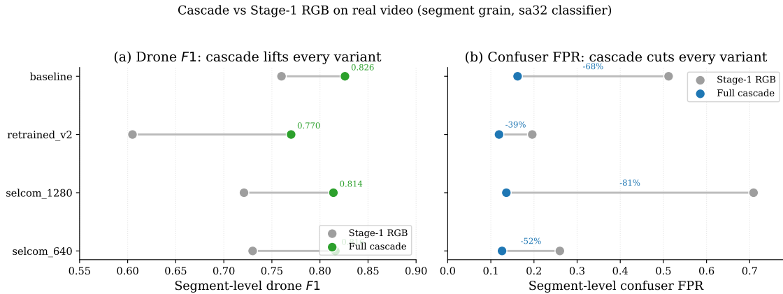
Figure 4.10: Design-evolution record (predecessor stack: baseline RGB, sa32 , alert-gated patch): segment-level drone F1 and confuser FPR, Stage-1 RGB (grey) versus the full cascade, on the real-video diagnostic. (a) The cascade lifts drone F1 for every variant. (b) It cuts confuser FPR by 39–81%. The production-stack re-run of this surface is Table 4.17.
