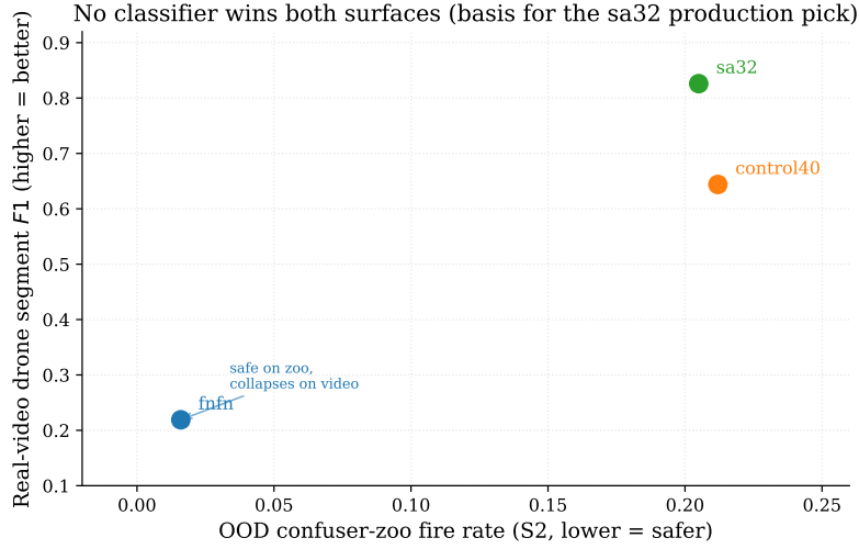
Figure 4.6: No trust classifier wins both surfaces. On the OOD confuser zoo fusion_no_fn_v1.1 is far the safest (S2 fire 0.016) but on real video it collapses drone F1 to 0.219; sa32 inverts the ranking, dominating real-video drone F1 (0.826) at a higher zoo fire (0.205). This surface reversal motivated the sa32 working pick, later superseded by the statistically-derived robust6/robust8 (Section 3.8.9) and the shipped no-reject robust8-nr (Section 4.1.4); sa32 ’s scene-statistic leakage (Section 3.8.9) lets it score partly by memorising surface identity, so its lead is not trusted to generalise.
