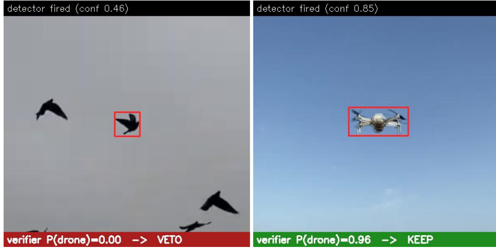
Figure 3.10: The confuser problem, and why a downstream filter solves it. Left : the production RGB detector ( ft4 ) fires on a bird amid its flock (red box, detector confidence 0.46). Right : it fires on a drone (confidence 0.85). The detector cannot tell them apart, but the feature-reuse filter reads the detector’s own internal features and assigns P(\text{drone}) = 0.00 to the bird (vetoed) and 0.96 to the drone (kept). This separation, not a better detector, is what the cascade provides.
