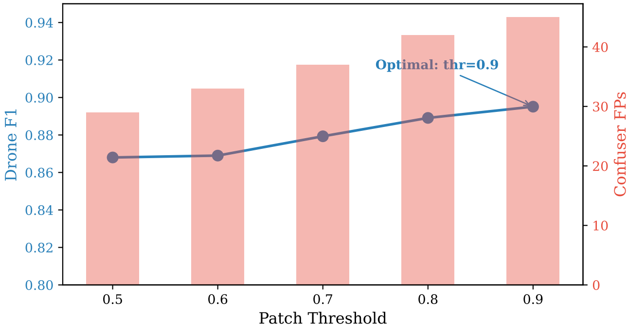
Patch Threshold Operating Point Selection (Svanström)
