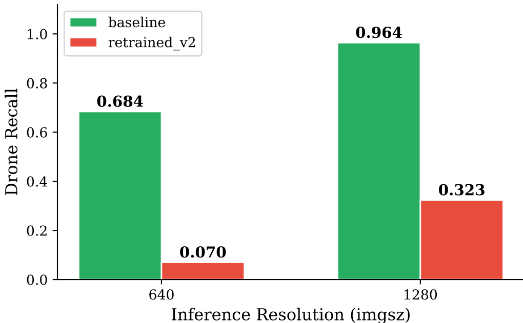
Svanström Drone Recall vs Resolution, per model (one harness: stride-7, n=4,102, IoP@0.5)
