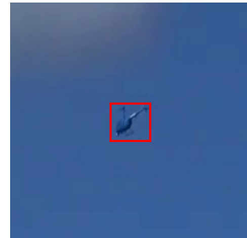
helicopter — det conf 0.85, filter P(\text{drone}) 0.009
