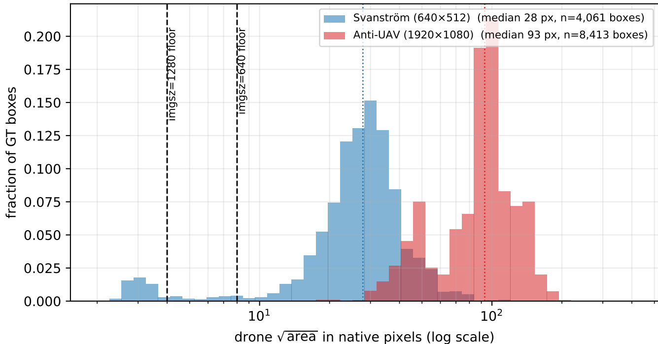
Drone size by dataset: why Svanström needs imgsz=1280
