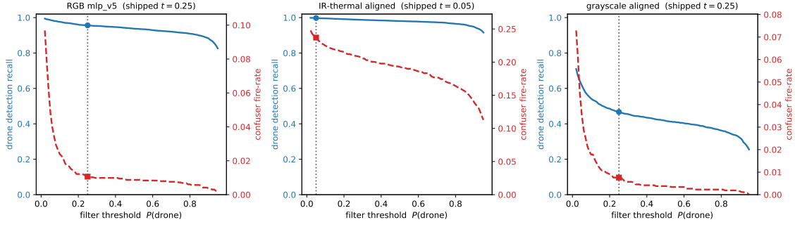
Figure 4.9: Filter operating points (detection level). For each confuser filter, drone detection recall (blue, left axis; fraction of GT-matched true-drone detections retained, pooled over the drone surfaces) and confuser fire-rate (red dashed, right axis; matching confuser surface) as the per-detection P(\text{drone}) threshold varies; the shipped point ( t = 0.25 RGB, 0.05 IR-thermal, 0.25 grayscale) is marked. RGB sits on a flat high-recall shoulder; the IR-thermal fire-rate is threshold-insensitive (the airplane coverage gap); the grayscale scaler trades recall steeply (the cross-domain fallback). Source: eval/filter_operating_sweep.py .
