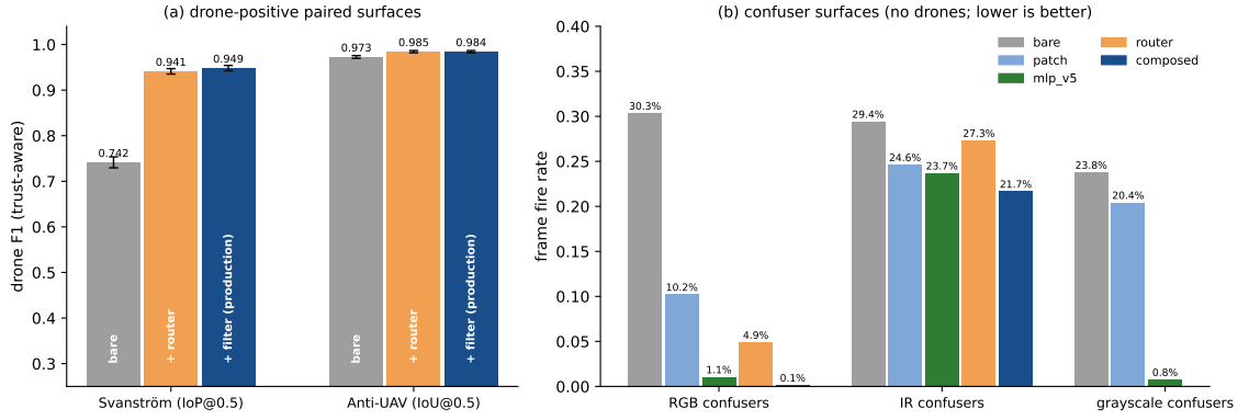
Figure 4.1: Pipeline ablation at a glance, drawn for the reject-class robust8 cascade (the strongest-suppression configuration; the shipped no-reject robust8-nr trades part of the confuser suppression for recall, Table 4.5). (a) Drone-positive paired surfaces: the router supplies most of the F1 lift and the filter finishes it; Anti-UAV confirms no-harm. Whiskers are 95% bootstrap CIs. (b) Confuser surfaces: bare \rightarrow patch \rightarrow mlp_v5 \rightarrow router \rightarrow composed frame fire rates, with near-total suppression on RGB (30.3% \rightarrow 0.15% composed) and grayscale (23.8% \rightarrow 0.8%) and measured resistance on thermal airplanes; the shipped no-reject stack delegates suppression to the filter alone and sits at 1.1% on RGB. Generated from tier1_results.json by thesis_eval/gen_ablation_figure.py .
