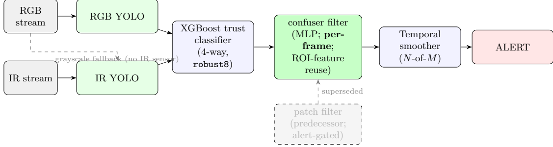
Figure 3.10: Multi-stage drone detection pipeline in the production composition: detectors, then the trust classifier, then the confuser filter. The order itself was ablated (Section 4.1): classifier-first is the recall-safe choice, within a point of the alternative. The production confuser filter is the distilled mlp_v5 , which runs per frame because it reuses the detectors’ already-computed ROI features rather than re-processing crops (Section 3.8.11). It supersedes the MobileNetV3 patch filter (greyed), which was expensive enough that it had to be alert-gated : consulted only when the temporal smoother was about to fire (Section 3.8.4).
