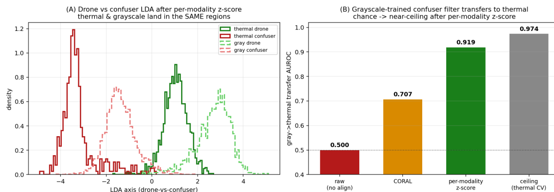
Figure 4.12: Grayscale↔thermal feature alignment in the IR detector. (A) After a per-modality z-score, thermal and grayscale drones land in the same region of the drone-vs-confuser discriminant axis, and likewise for confusers: the modalities are interchangeable up to an affine offset. (B) Grayscale-trained confuser-filter transfer to thermal rises from chance (0.500) to near the within-thermal ceiling (0.919 vs 0.974) once the offset is removed; CORAL (0.707) under-performs the simpler z-score.
