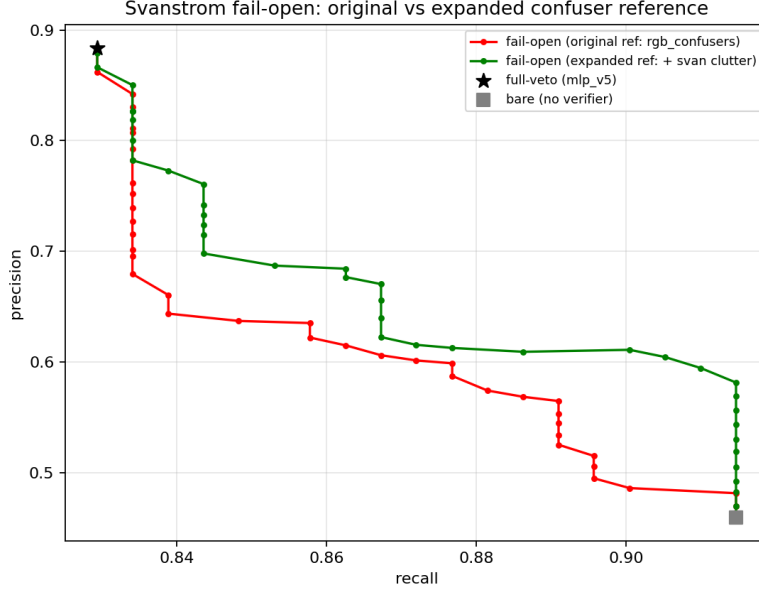
Figure 4.8: Why fail-open is not adopted: the recall/precision frontier on Svanström for the fail-open gate with the original rgb_confusers reference (red) versus a reference expanded with held-out Svanström clutter (green), against the full-veto operating point (star) and the bare detector (square). The full-veto point dominates at high recall; the trade is partly calibration and partly fundamental. Source: eval/failopen_expanded_ref.py .
