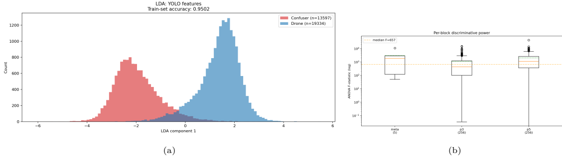
Figure 4.10: Model MRI of the FT4 detector’s fused p3+p5 ROI features on the shipped 32,931-detection corpus. (a) The linear-discriminant projection separates drone (blue) from confuser (red) into two cleanly-resolved peaks at \approx 95\% single-threshold accuracy. (b) Per-block ANOVA F -statistic: p5 is the dominant discriminative layer (max F = 42,346 , mean 2,006), ahead of p3 and the detection metadata; the confidence scalar ranks only 6th.
