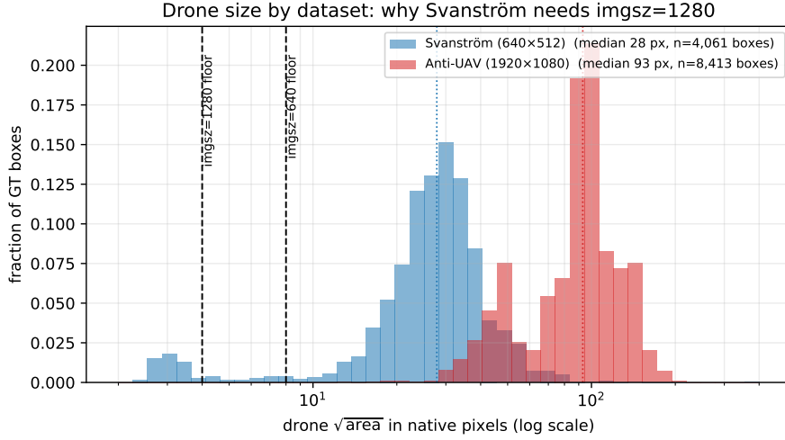
Figure 3.5: Drone size by dataset: the distribution of ground-truth box sizes ( \sqrt{\text{area}} in native pixels; a sample of up to 9,000 label files per dataset, n in the legend counts boxes, not frames; each histogram shows the fraction of that dataset’s boxes per bin). Svanström drones (median 28 px) sit close above the YOLOv26n imgsz=640 resolvable floor ( \sqrt{\text{area}} \approx 8 px), with a visible sub-floor tail; small targets near the floor are where detection degrades long before the hard limit, which is why Svanström recall degrades sharply at imgsz=640 (baseline 0.964 \rightarrow 0.684) and resolves at imgsz=1280 (floor \approx 4 px; Section 3.8.6). Anti-UAV drones (median 93 px) are an order of magnitude larger and supra-floor at either resolution.
