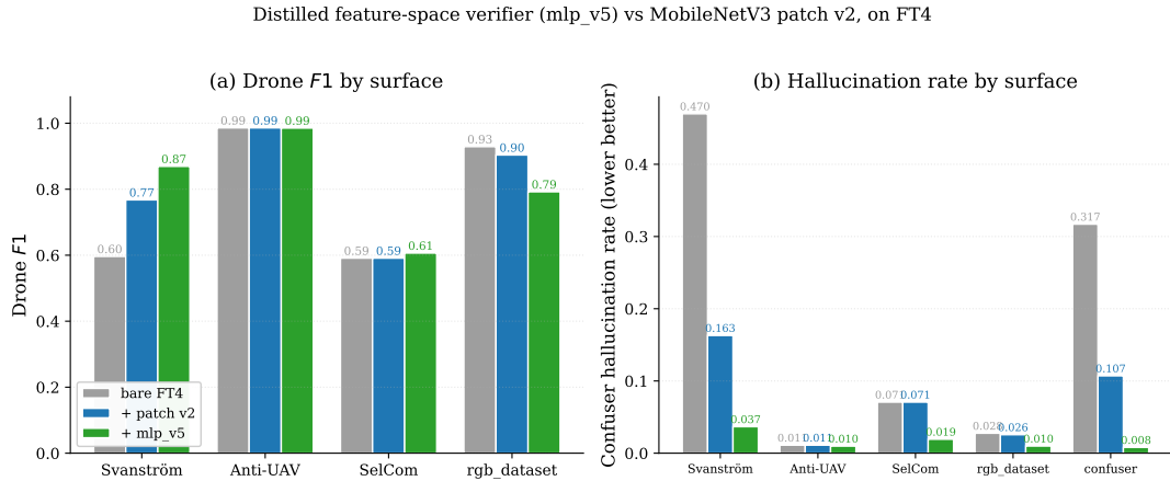
Figure 4.7: Feature-reuse filter ( mlp_v5 , green) vs the MobileNetV3 patch filter (v2, blue) and the bare FT4 detector (grey), per evaluation surface. (a) Drone F1 : mlp_v5 wins Svanström and SelCom, ties saturated Anti-UAV, and regresses on the photo-style rgb_dataset split. (b) Confuser hallucination rate: lowest on every surface. Generated from knowledge/evals.csv .
