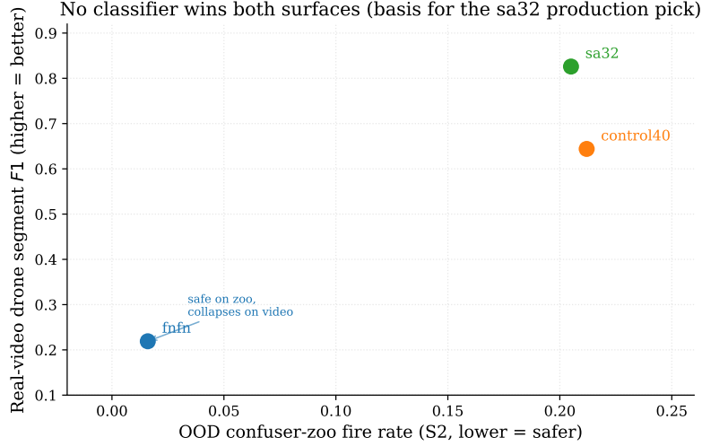
Figure 4.5: No trust classifier wins both surfaces. On the OOD confuser zoo fusion_no_fn_v1.1 is far the safest (S2 fire 0.016) but on real video it collapses drone F1 to 0.219; sa32 inverts the ranking, dominating real-video drone F1 (0.826) at a higher zoo fire (0.205). This surface reversal motivated the sa32 working pick, later superseded by the statistically-derived robust6/robust8 (Section 3.8.9) and the shipped no-reject robust8-nr (Section 4.3.3).
