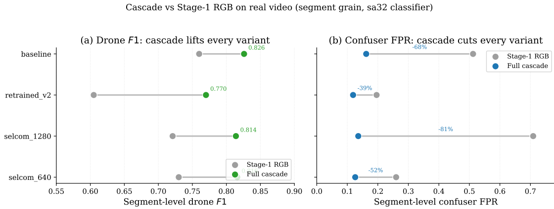
Figure 4.2: Design-evolution record (predecessor stack: baseline RGB, sa32 , alert-gated patch): segment-level drone F1 and confuser FPR, Stage-1 RGB (grey) versus the full cascade, on the real-video diagnostic. (a) The cascade lifts drone F1 for every variant. (b) It cuts confuser FPR by 39–81%. The production-stack re-run of this surface is Table 4.12.
