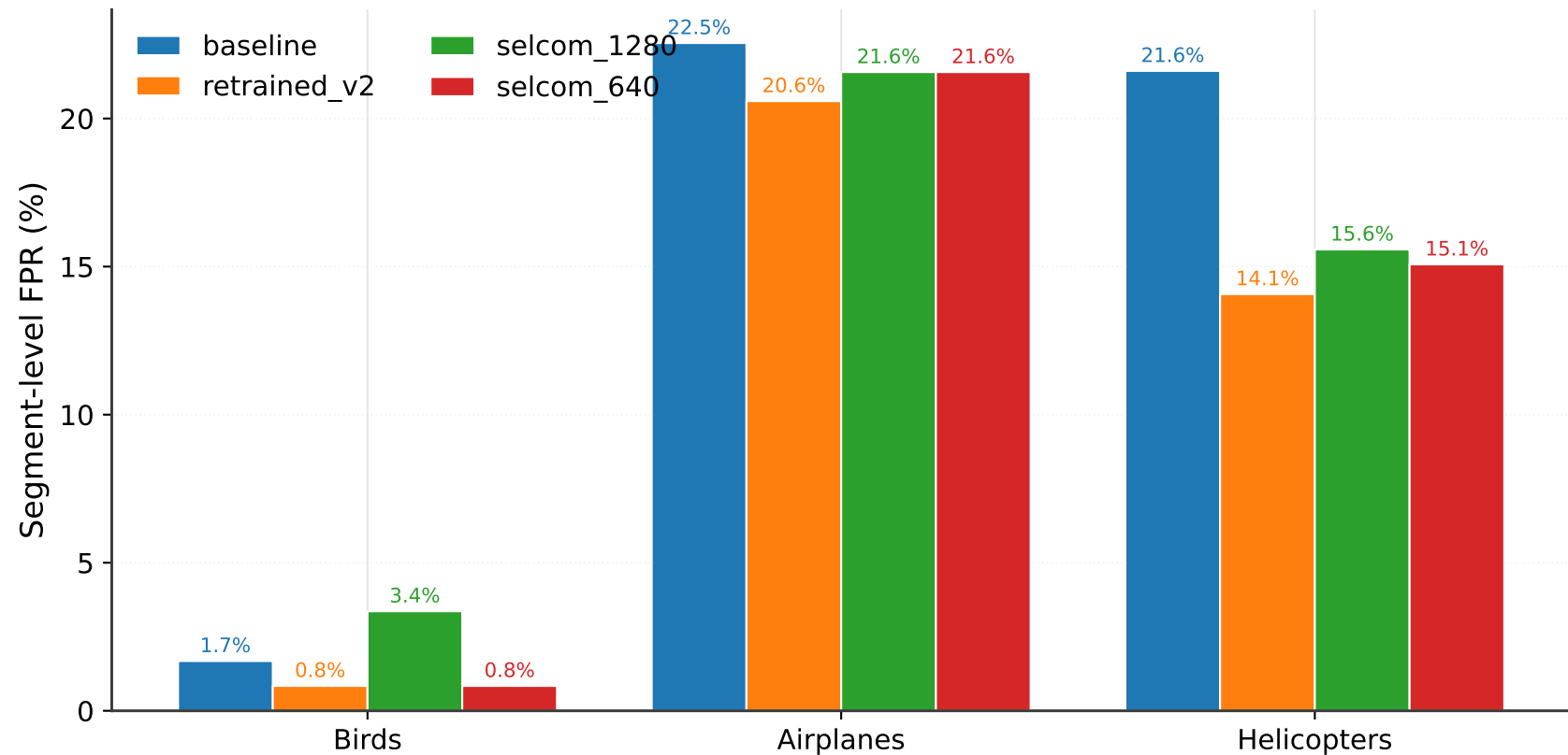
Per-category cascade confuser FPR on real-video diagnostic (sa32)
