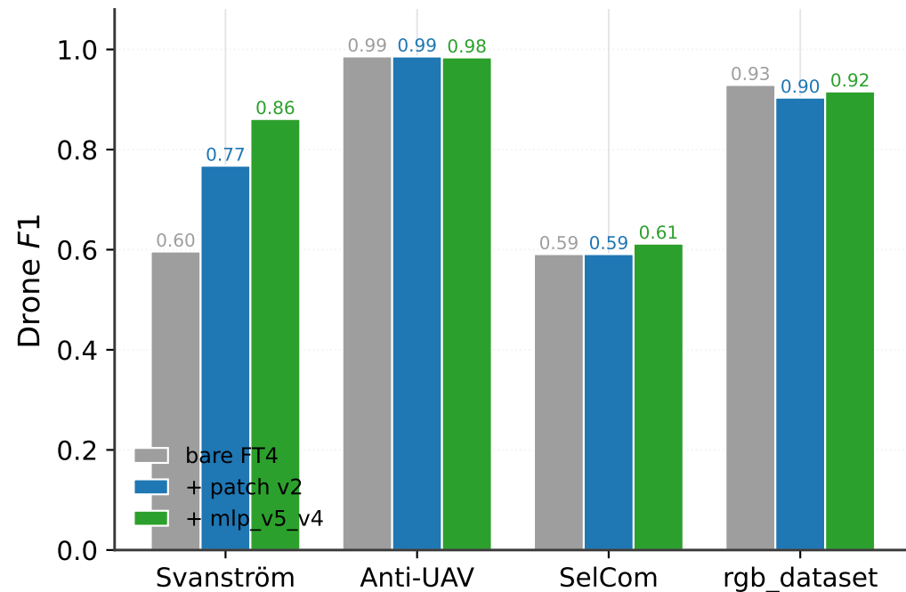
(a) Drone F1 by surface
