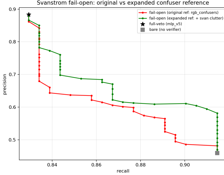
Figure 4.8: Design-history: the recall/precision frontier on Svanström for the no-retrain fail-open gate (with the original rgb_confusers reference, red, versus a reference expanded with held-out Svanström clutter, green), against the full-veto operating point (star) and the bare detector (square). This gate was the candidate fix before the bird-split re-mine closed the coverage gap directly; it is retained only as the record of why a calibration patch was inferior to fixing the training coverage. Source: eval/failopen_expanded_ref.py .
