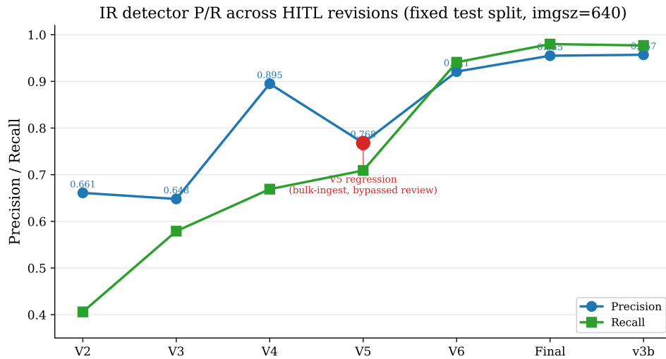
Figure 4.3: IR detector P/R trajectory across the five numbered revisions (V2–V6) plus the Final retrain and production v3b , on the fixed IR_dset_final test split. The V5 regression (precision 0.895 \rightarrow 0.768) is recovered by V6 and the production v3b .
