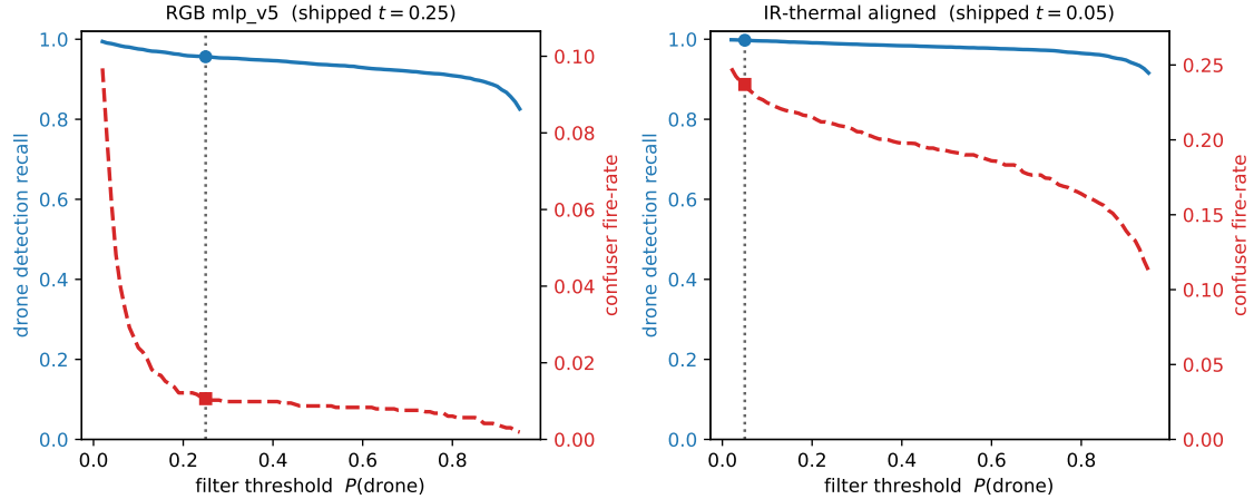
Figure 4.9: Filter operating points (detection level). For each production confuser filter, drone detection recall (blue, left axis; fraction of GT-matched true-drone detections retained, pooled over the drone surfaces) and confuser fire-rate (red dashed, right axis; matching confuser surface) as the per-detection P(\text{drone}) threshold varies; the shipped point ( t = 0.25 RGB, 0.05 IR-thermal) is marked. RGB sits on a flat high-recall shoulder; the thermal-native head now suppresses thermal confusers (fire falls with the threshold; the residual is the airplane-like in-distribution fraction). Source: eval/filter_operating_sweep.py .
