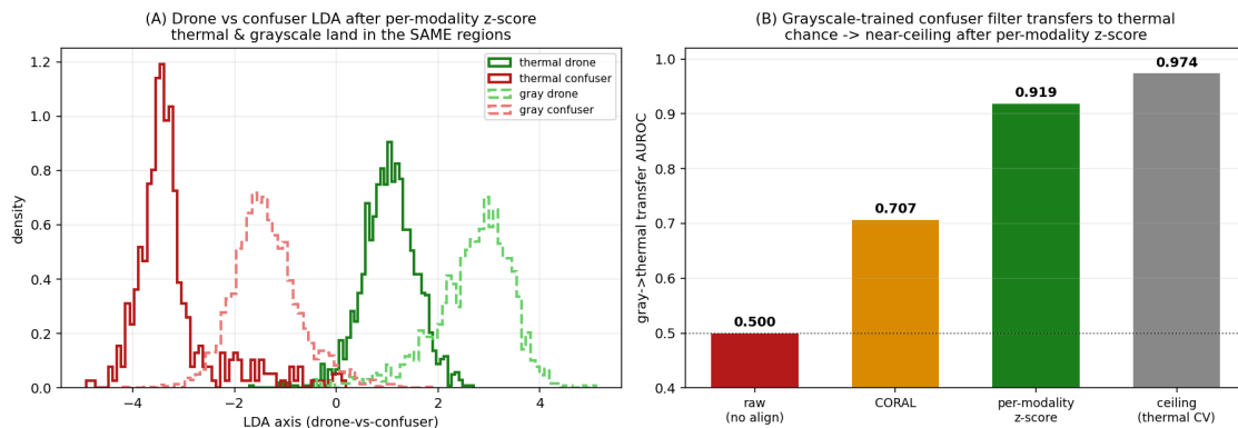
Figure 4.12: Grayscale \leftrightarrow thermal feature alignment in the IR detector. (A) After a per-modality z-score, thermal and grayscale drones land in the same region of the drone-vs-confuser discriminant axis, and likewise for confusers: the modalities are interchangeable up to an affine offset. (B) Grayscale-trained confuser-filter transfer to thermal rises from chance (0.500) to near the within-thermal ceiling (0.919 vs 0.974) once the offset is removed; CORAL (0.707) under-performs the simpler z-score.
