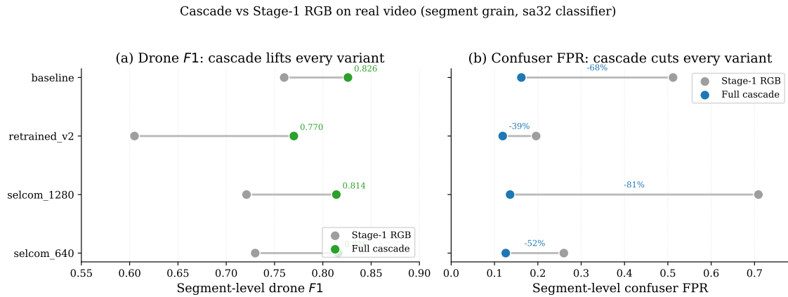
Figure 4.6: Design-evolution record (predecessor stack: baseline RGB, sa32, alert-gated patch): segment-level drone F1 and confuser FPR, Stage-1 RGB (grey) versus the full cascade, on the real-video diagnostic. (a) The cascade lifts drone F1 for every variant. (b) It cuts confuser FPR by 39–81%. The production-stack re-run of this surface is Table 4.11.
