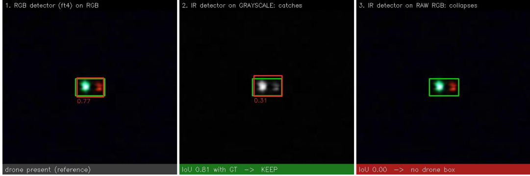
Figure 4.7: Cross-modal transfer, illustrated on one Anti-UAV night frame (each panel cropped around the drone). Left : the production RGB detector ( ft4 ) on the RGB frame, for reference. Middle : the IR detector ( v3b ), trained zero-shot on thermal only, applied to the grayscale-converted frame; it lands the drone (IoU 0.81 with the green GT box). Right : the same IR detector on the raw 3-channel RGB collapses (IoU 0.00, no box). The transfer is carried by the single-channel intensity input; the colour information that distinguishes thermal from visible is what breaks it.
